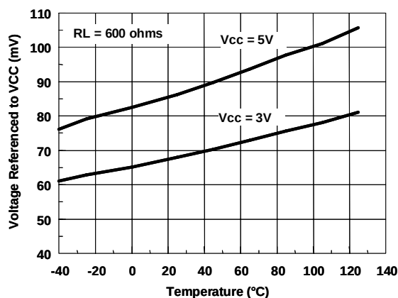
Figure 8. High level output voltage vs. temperature
