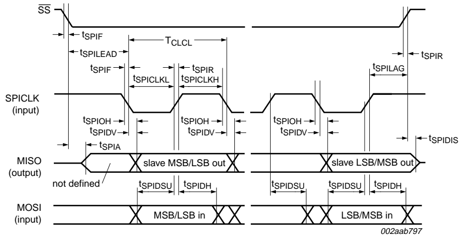
Fig 21. SPI slave timing (Mode 3)
