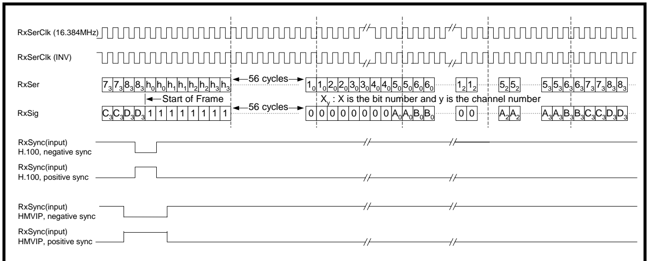
FIGURE 70. TIMING SIGNAL WEHN THE RECEIVE FRAMER IS RUNNING AT H MVIP AND H100 16.384MHz MODE
