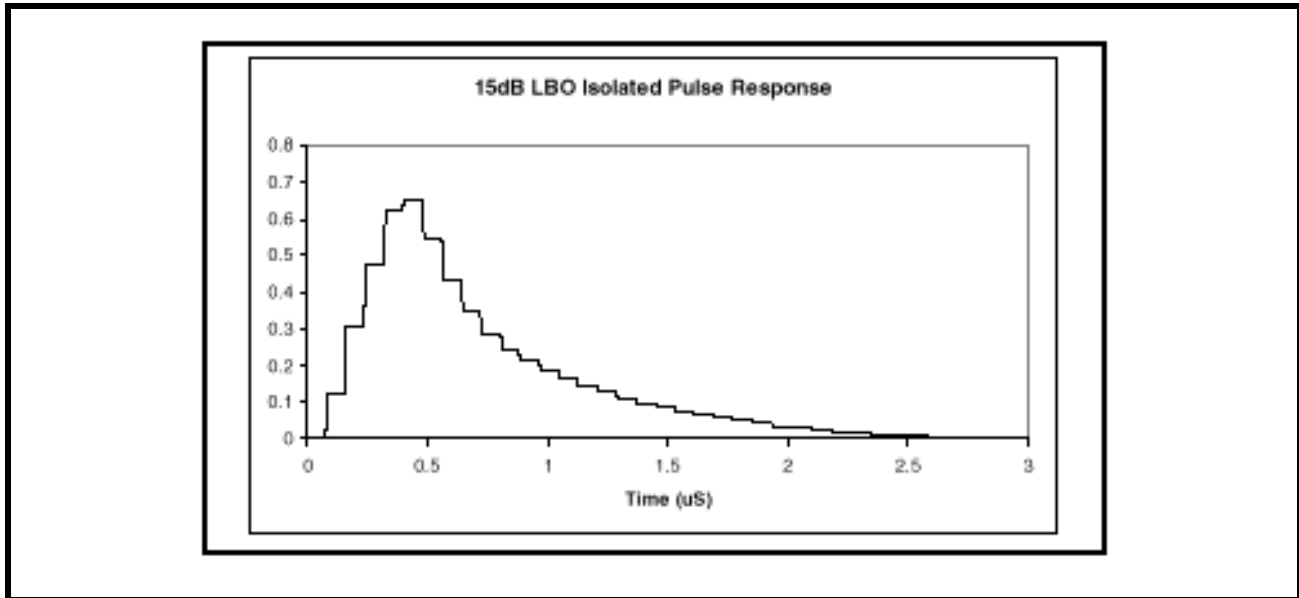
FIGURE 47. LONG HAUL LINE BUILD OUT WITH -15dB ATTENUATION
