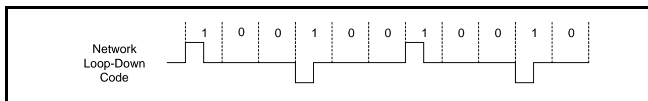
FIGURE 45. NETWORK LOOP DOWN CODE GENERATION
