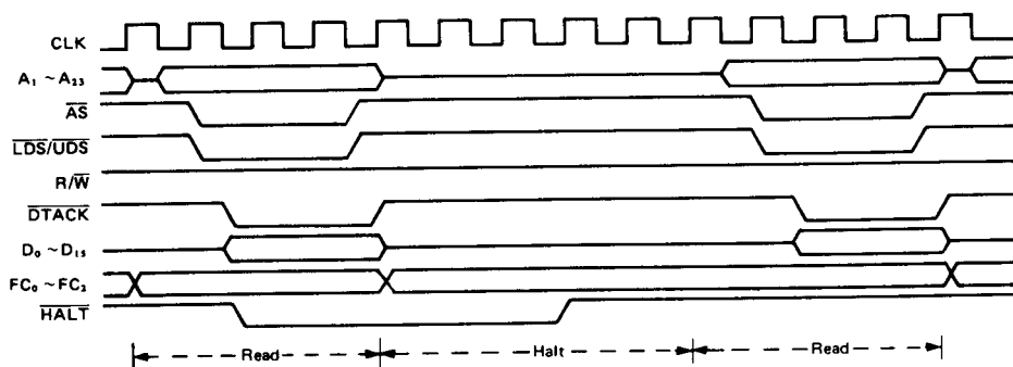
Figure 33 Halt Signal Timing Characteristics
