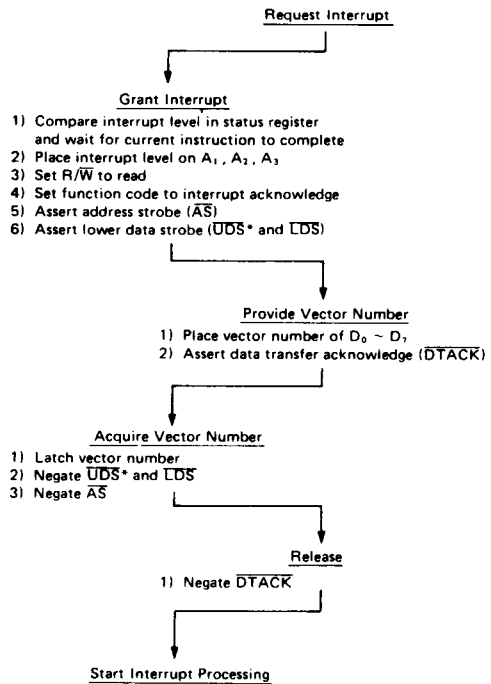
Figure 42 Interrupt Acknowledge Sequence Flow Chart
