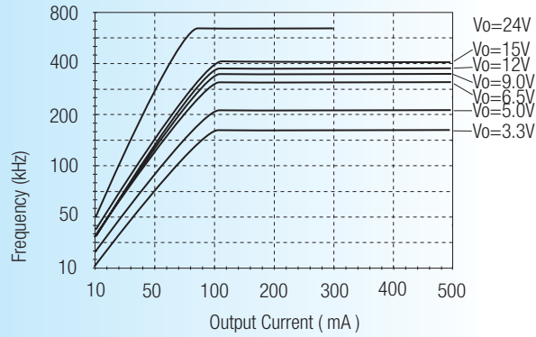
Switching Frequency Vs Load (Vin=30~72V)
