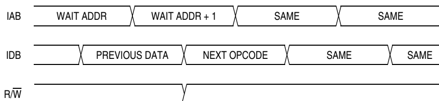
Figure 16-15. Wait Mode Entry Timing
