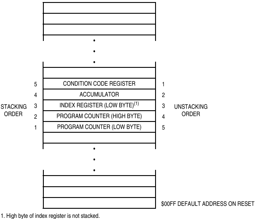
Figure 14-3. Interrupt Stacking Order
