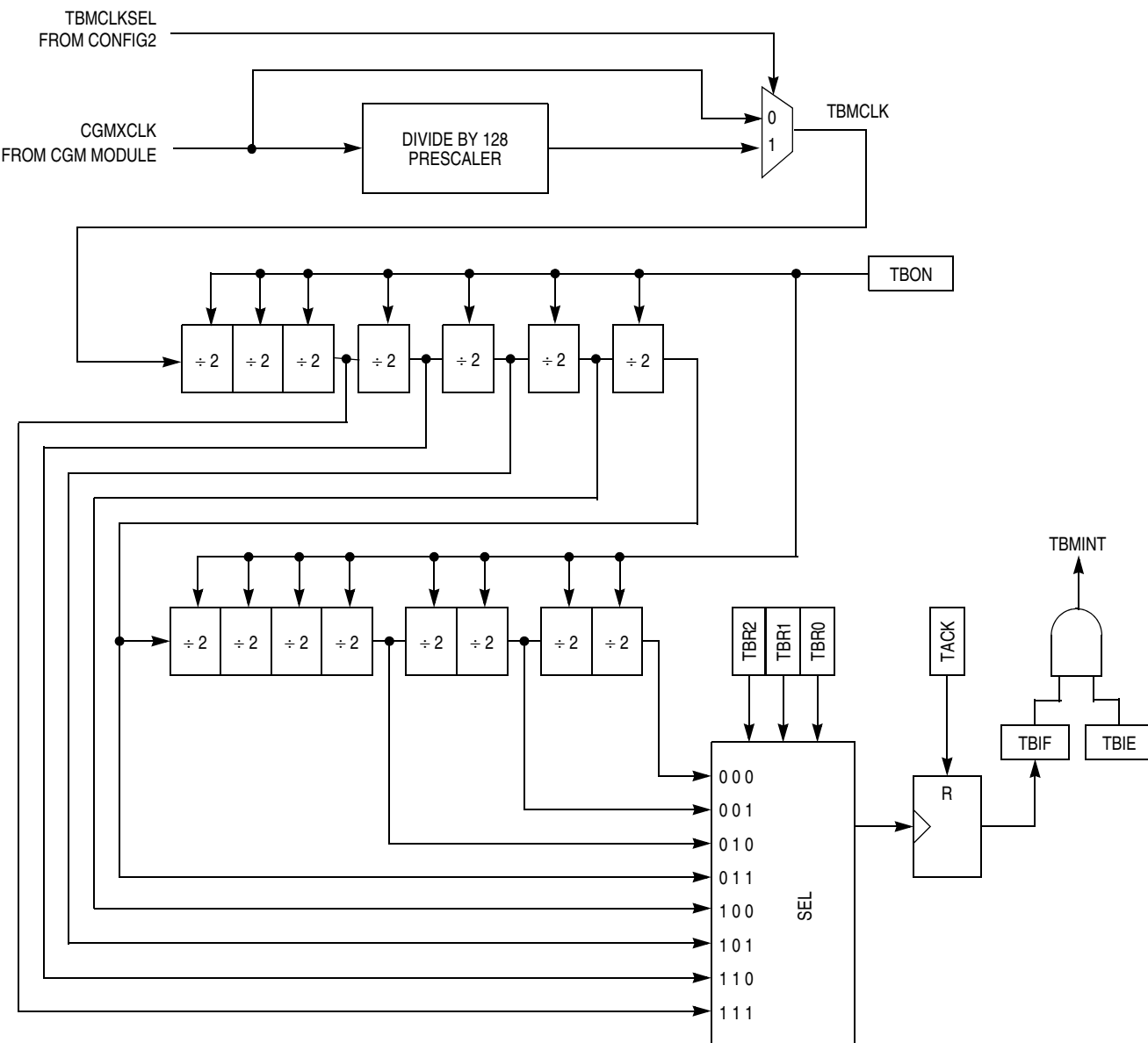
Figure 18-1. Timebase Block Diagram
