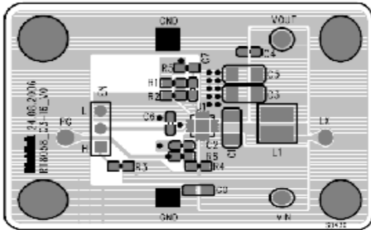
Figure 3. Top Layer
