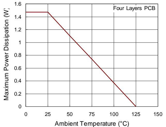
Figure 2. Derating Curves for RT8058 Package
