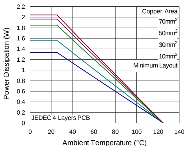
Figure 4. De-rating Curves
