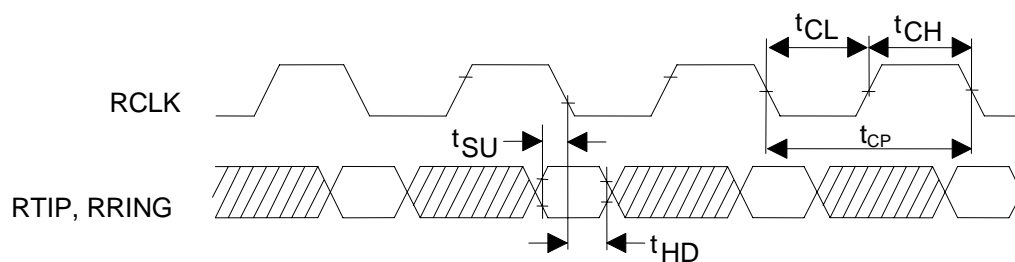
Figure 12-7. Receive Framer Timing—Line Side
