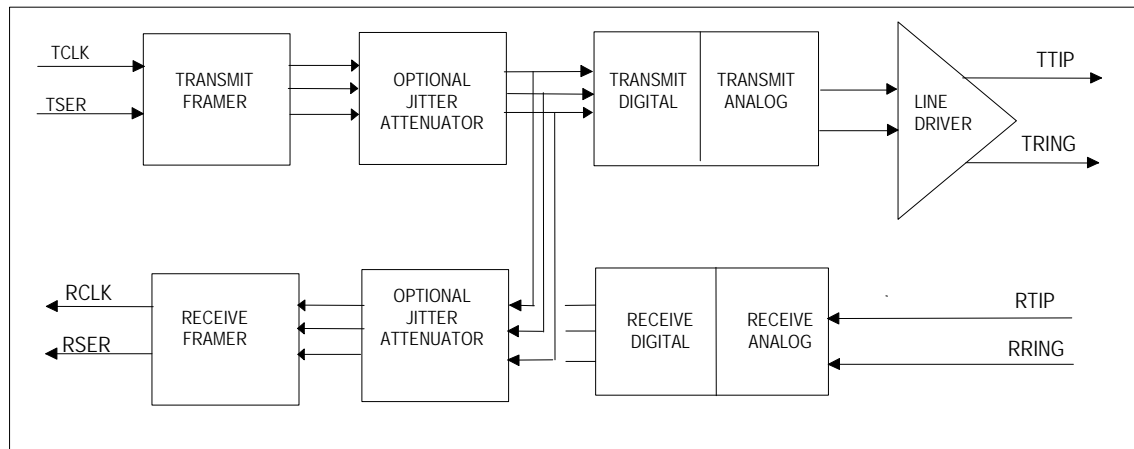
Figure 8-17. Local Loopback
