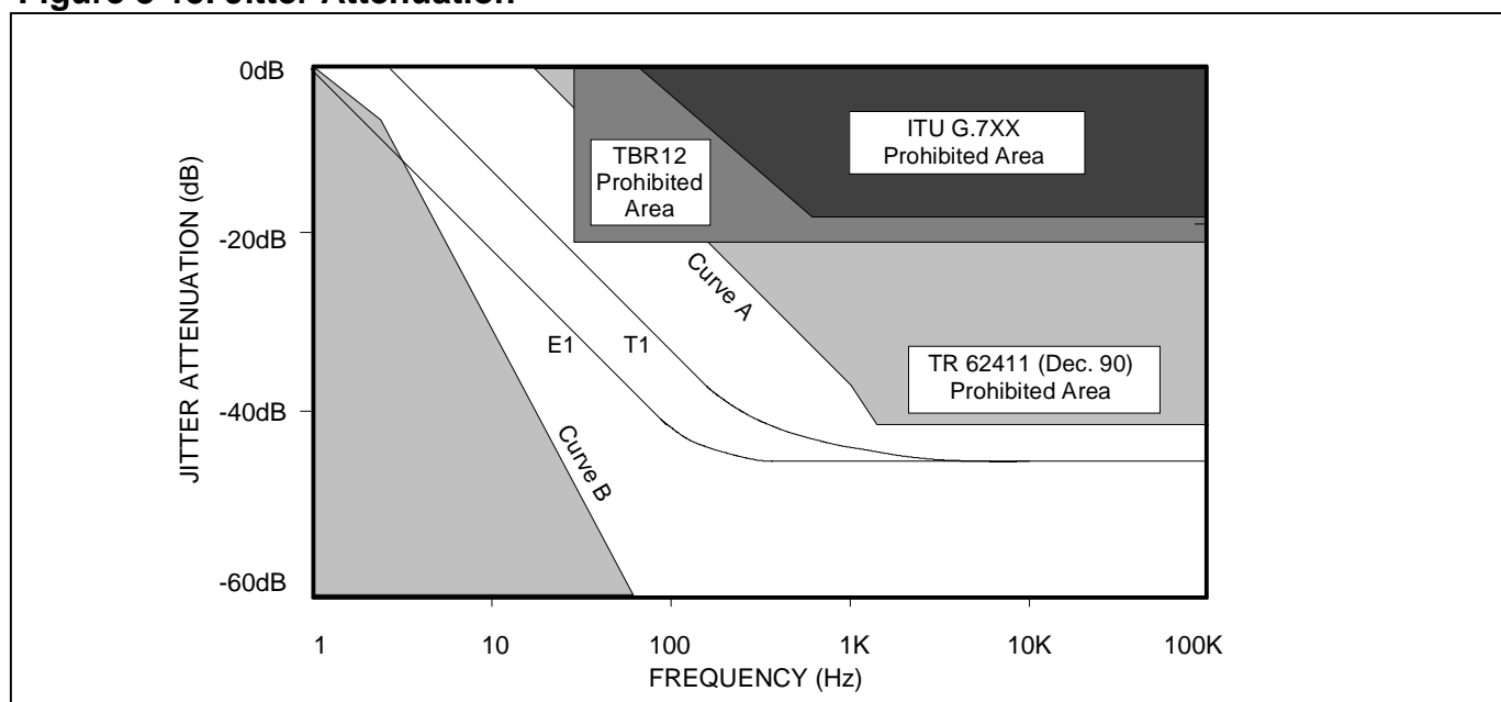
Figure 8-15. Jitter Attenuation
