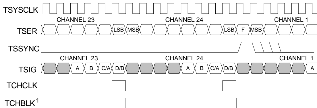
Figure 10-11. T1 Transmit-Side 1.544MHz Boundary Timing (Elastic Store Enabled)
