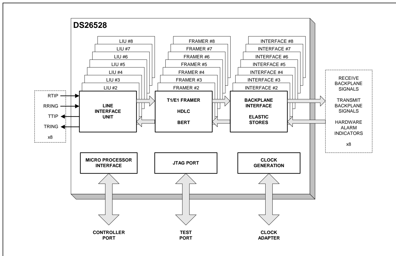
Figure 6-1. Block Diagram
