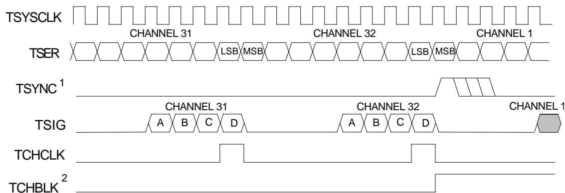
Figure 10-22. E1 Transmit-Side 2.048MHz Boundary Timing (Elastic Store Enabled)
