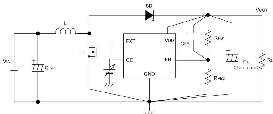
Circuit 2. XC6367B, XC6368B
