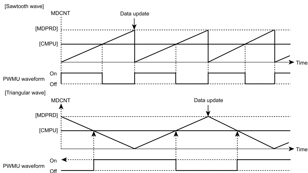
Figure 13-9 PWM Waveforms
