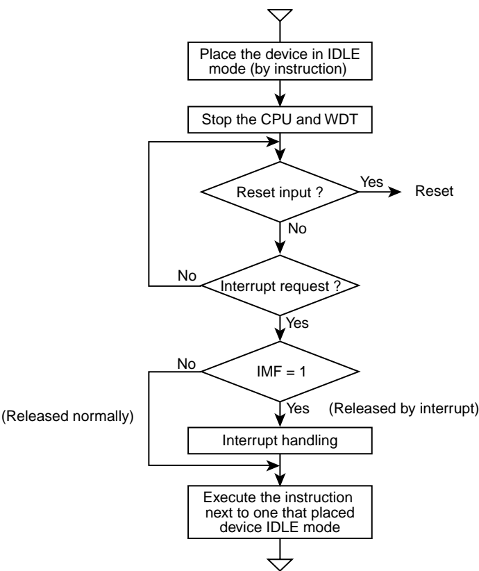
Figure 2-10 IDLE Mode
