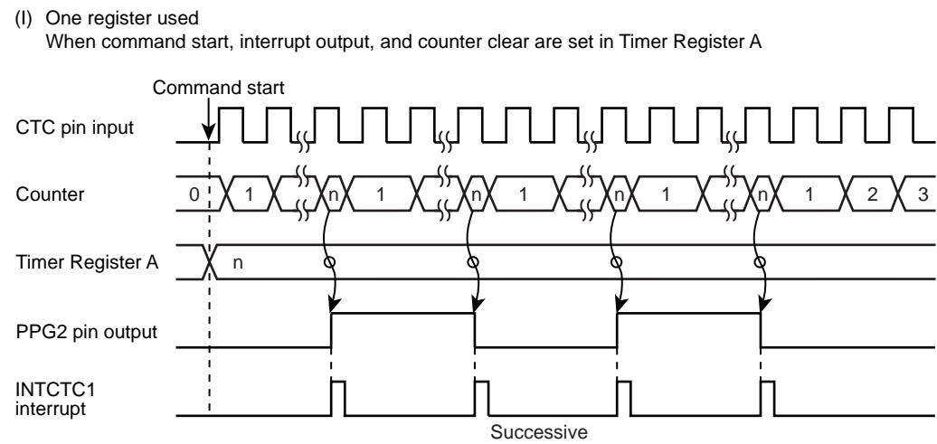
Figure 9-6 PPG Output Mode Timing Chart
