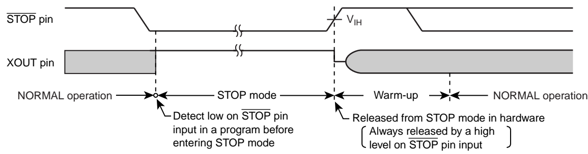
Figure 2-7 Released from STOP Mode by Level
