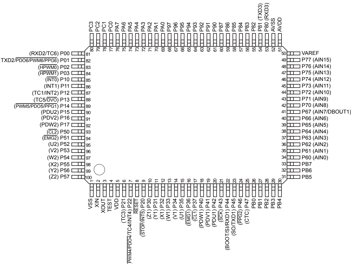
Figure 1-1 Pin Assignment
