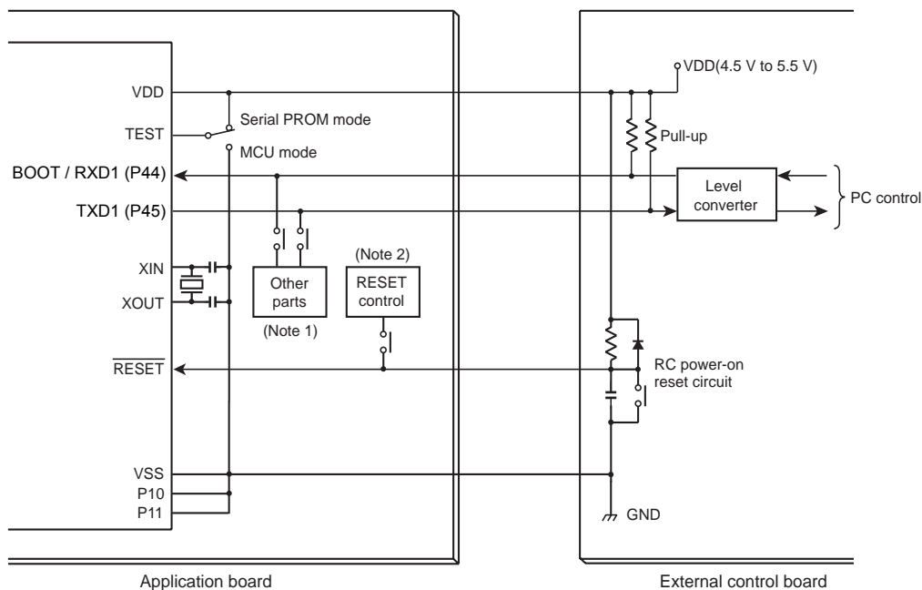
Figure 20-3 Example Connection for On-Board Writing
