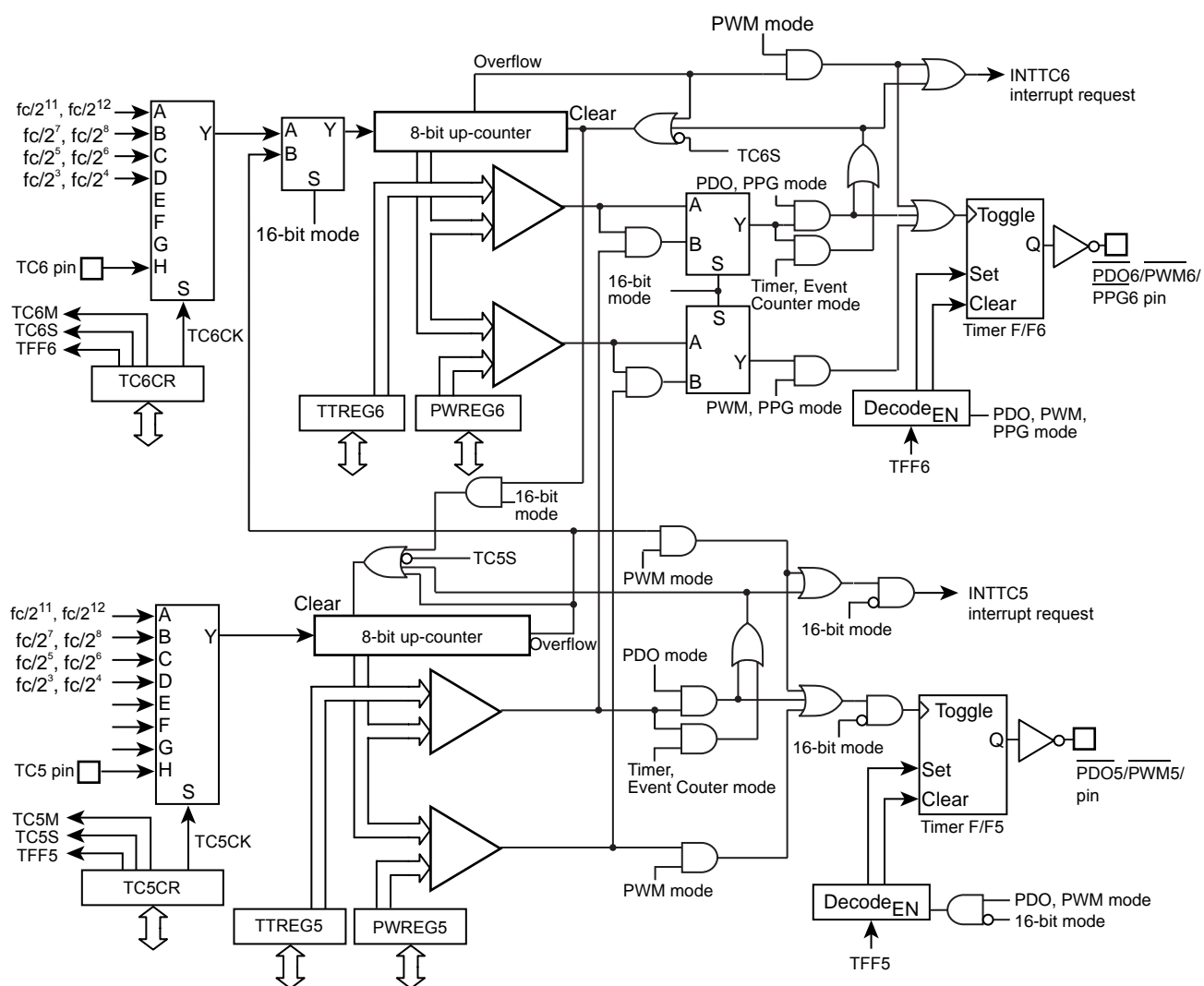
Figure 12-1 8-Bit TimerCounter 5, 6
