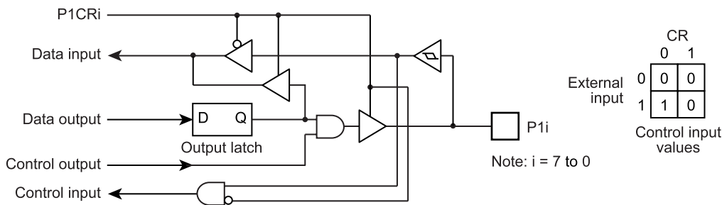
Figure 5-3 Port P1
