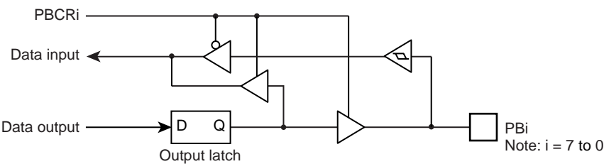
Figure 5-13 Port PB
