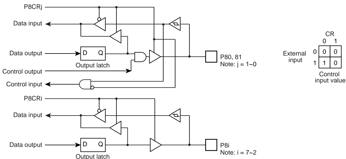
Figure 5-10 Port P8
