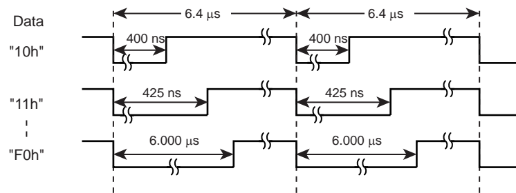
Figure 18-3 7-Bit Mode
