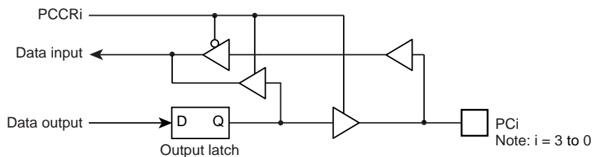
Figure 5-14 Port PC
