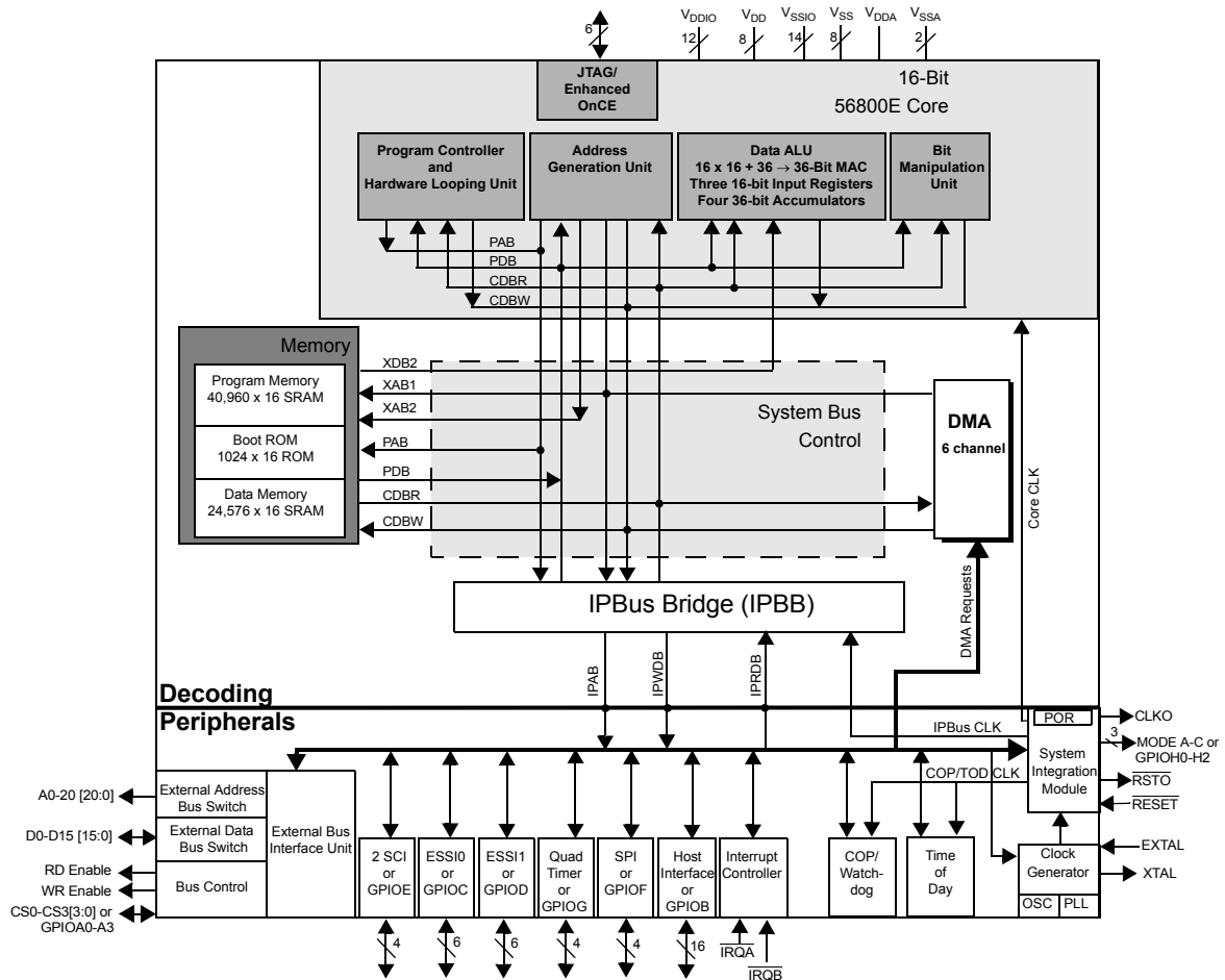
56858 Block Diagram
