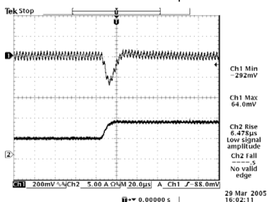
50% to 100% load 12 Vdc Input 5 Vdc Output
