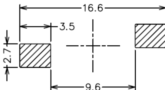
Soldering patterns
