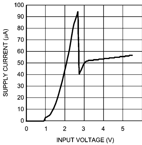
Supply Current vs Input Voltage
