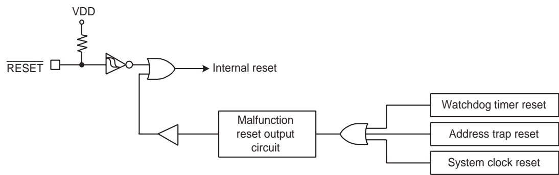
Figure 2-15 Reset Circuit
