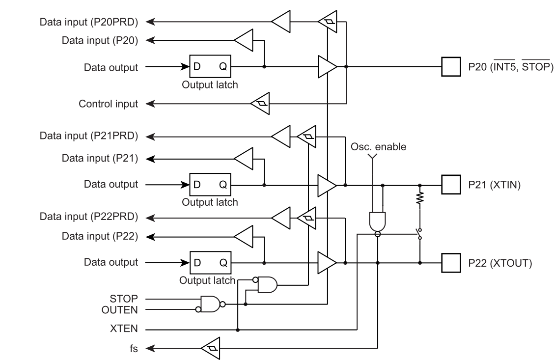
Figure 5-4 P2 Port
