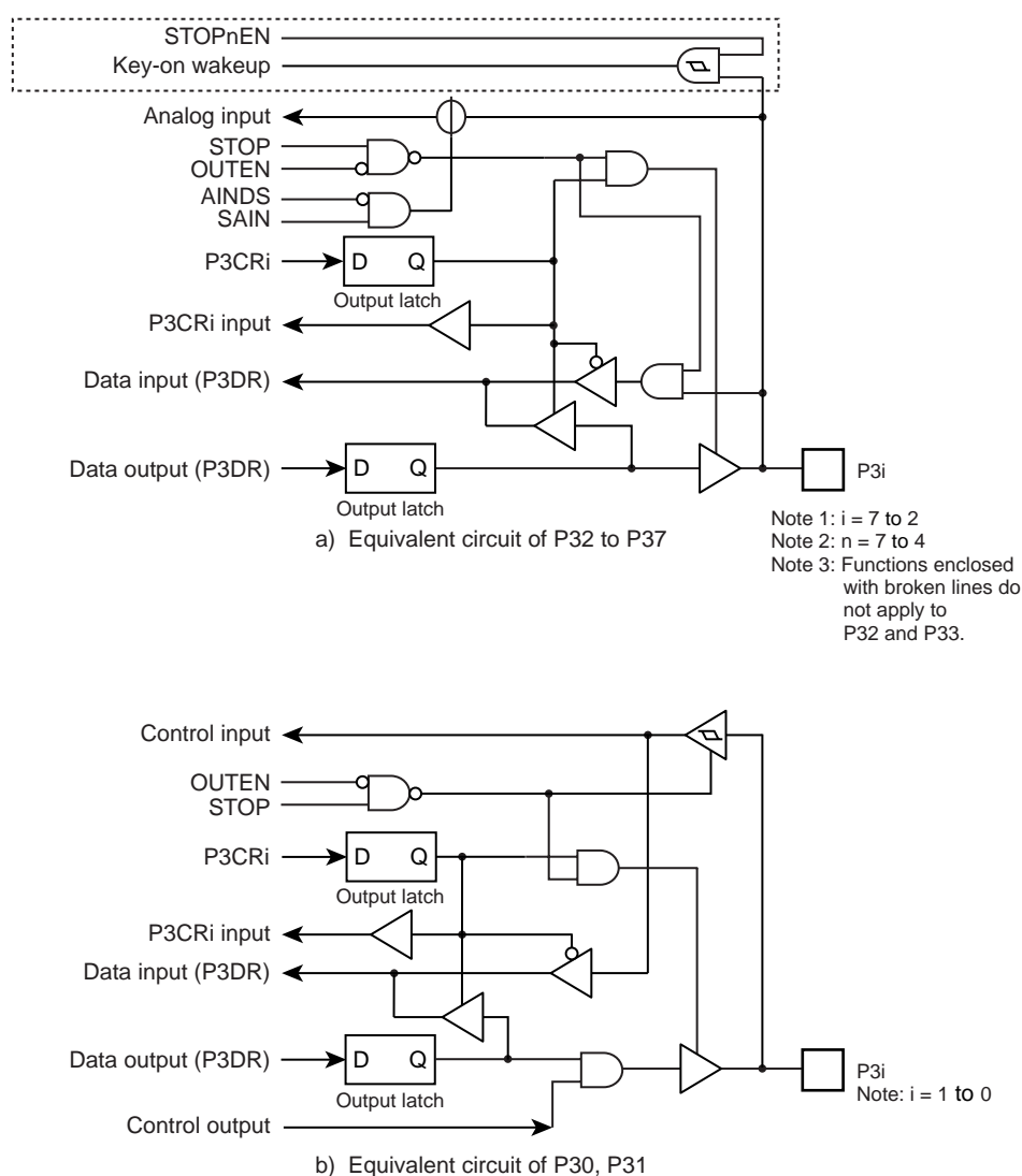
Figure 5-5 P3 Port
