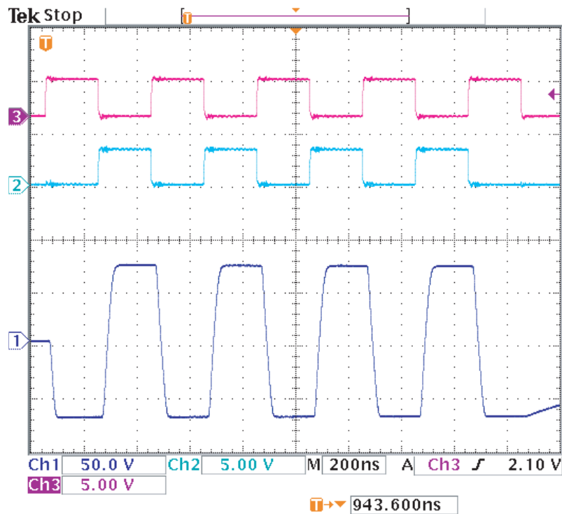
Figure 4: NIN, PIN and OUTPUT at 2.5MHz, V_{DD} = +9.0V , (V_{PP} - V_{PF}) = +9.0V , (V_{NF} - V_{NN}) = +9.0V , V_{PP}/V_{NN} = +/- 75V , Load = 330pF//2.49k \Omega , MC0 = MC1 = 1
