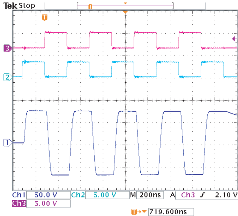
Figure 3: NIN, PIN and OUTPUT at 2.5MHz, V_{DD} = +9.0V , (V_{PP} - V_{PF}) = +9.0V , (V_{NF} - V_{NN}) = +9.0V , V_{PP}/V_{NN} = +/- 75V , Load = 330pF//2.49k \Omega , MC0 = MC1 = 1
