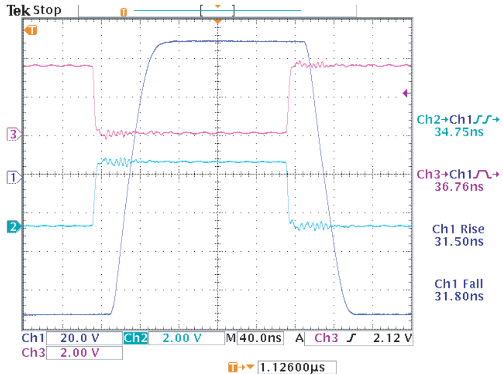
Figure 5: t_d/t_{df} = 20/20.5ns , t_r/t_f = 31.5/31.8ns , V_{DD} = +9.0V , (V_{PP} - V_{PF}) = +9.0V , (V_{NF} - V_{NN}) = +9.0V , V_{PP}/V_{NN} = +/- 75V , Load = 330pF//2.49k\Omega , MC0 = MC1 = 1
