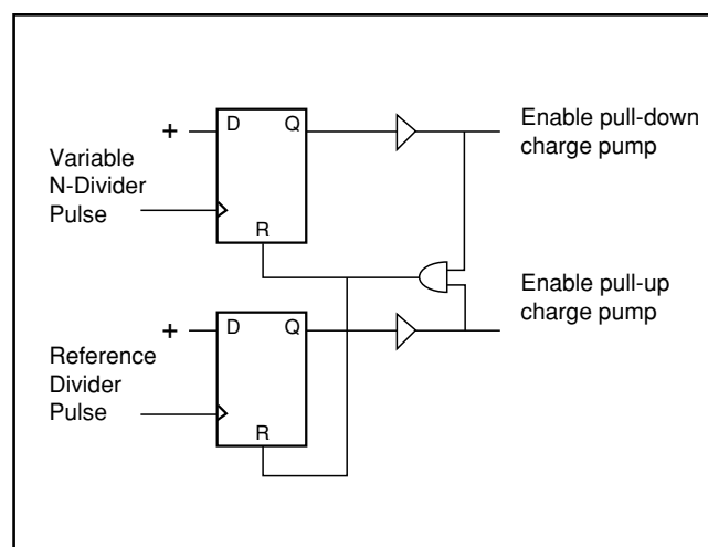
Figure 3 - Auxiliary phase detector
