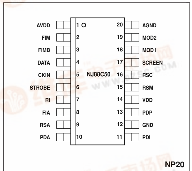
Figure 1 - Pin assignment
