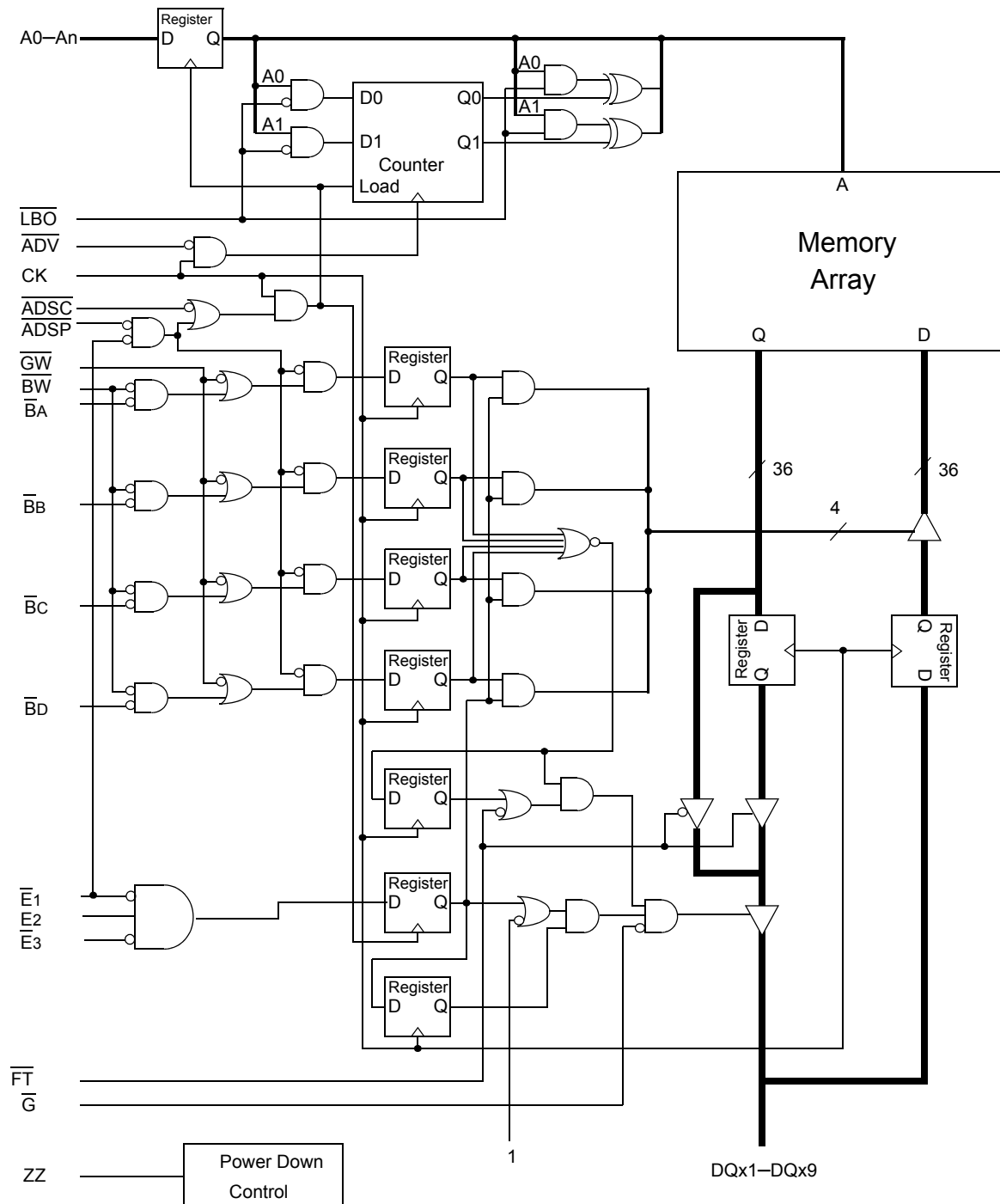
GS88018/32/36B Block Diagram
