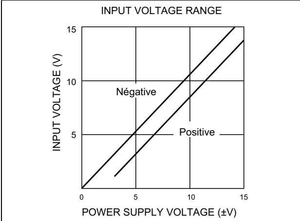
Figure 10. Input voltage range
