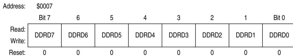
Figure 16-13. Data Direction Register D (DDRD)
