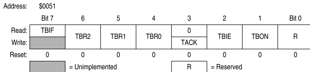
Figure 10-2. Timebase Control Register (TBCR)
