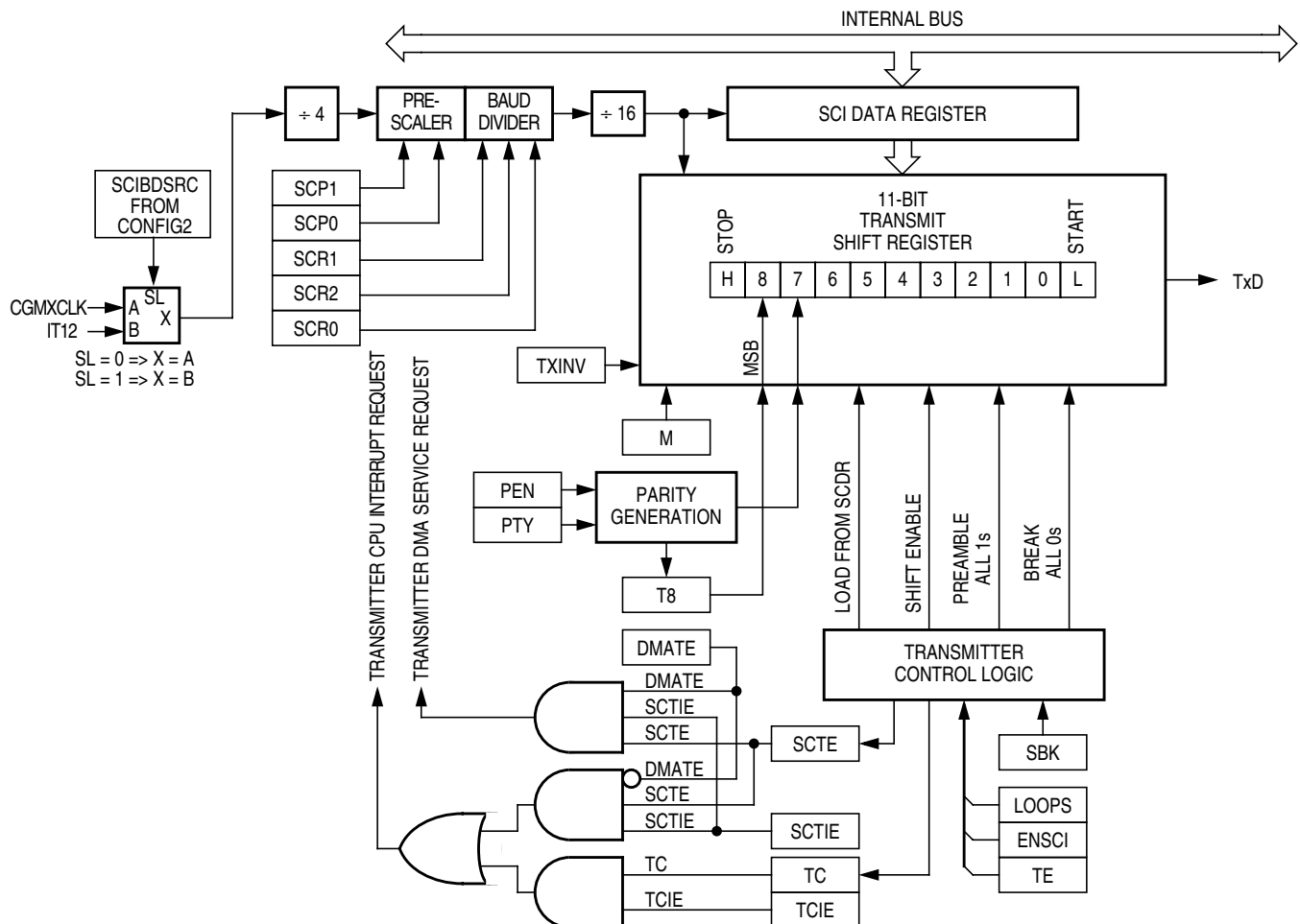
Figure 11-4. SCI Transmitter
