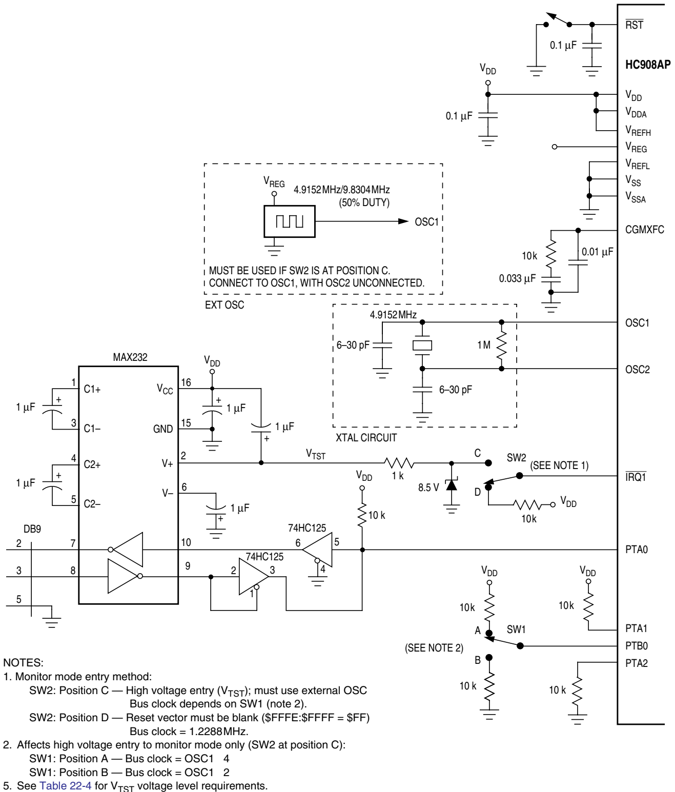
Figure 8-1. Monitor Mode Circuit
