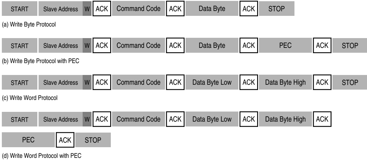
Figure 14-16. Write Byte/Word
