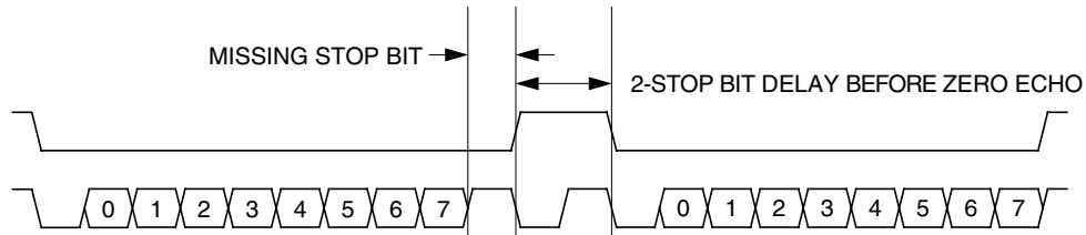
Figure 8-4. Break Transaction
