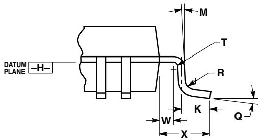
DETAIL C
