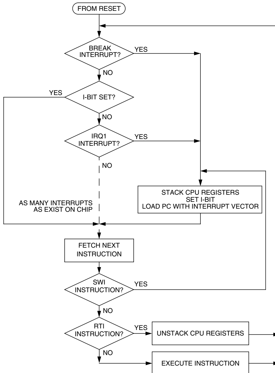
Figure 7-10. Interrupt Processing
