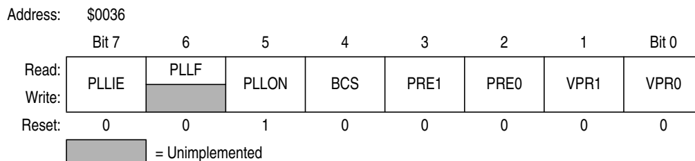
Figure 6-4. PLL Control Register (PCTL)
