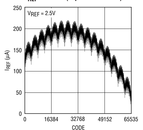
IREF vs Code (Bipolar LTC2642)
