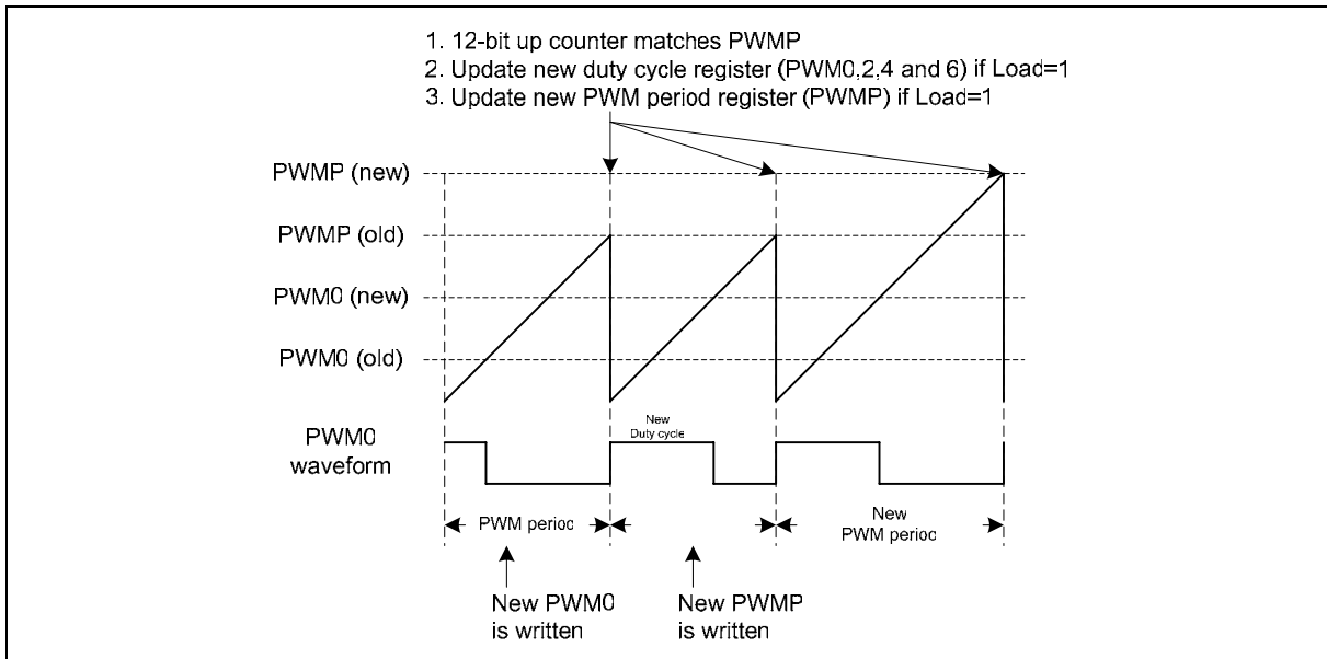
Figure 14-16: Edge-Aligned PWM
