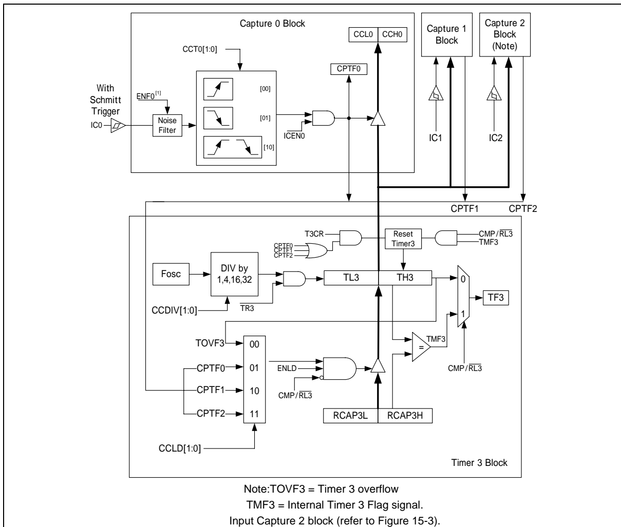
Figure 15-2: Timer3/Capture/Compare/Reload modules
