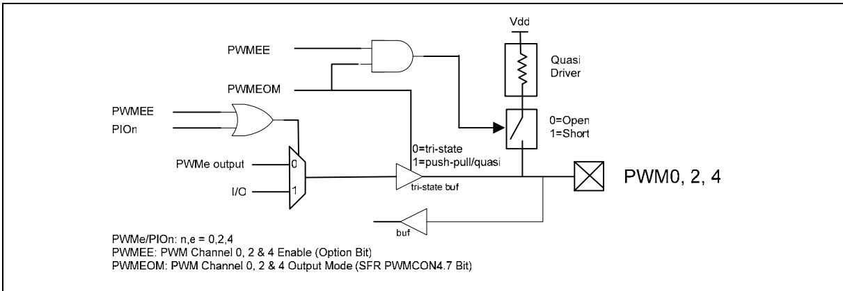
Figure 14-3: PWM0, 2 & 4 I/O pins
