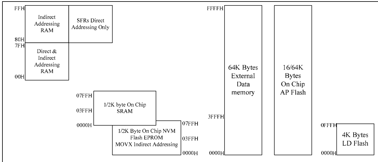
Figure 6-1: W79E22X SERIES Memory Map
