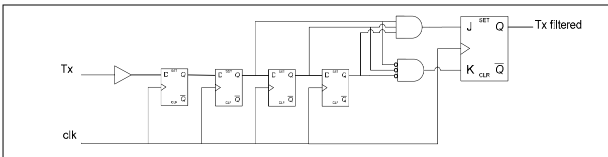
Figure 15-1: Noise Filter
