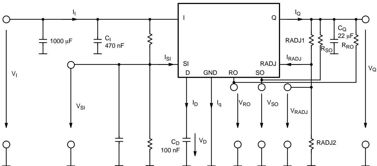
Figure 2. Measuring Circuit
