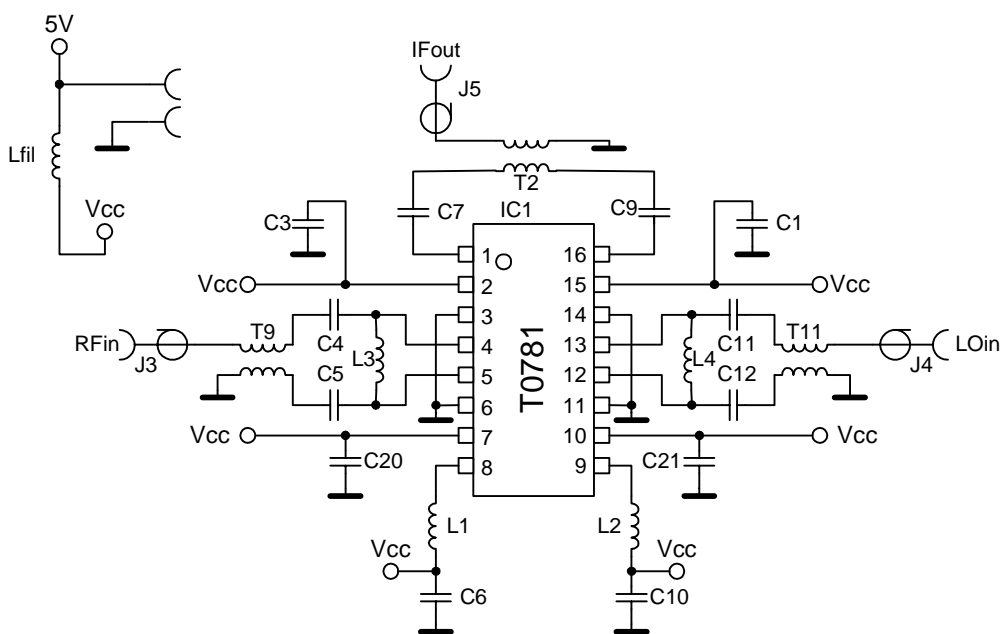
Figure 23. 1700 MHz to 2000 MHz Application Schematic (Differential Drive)
