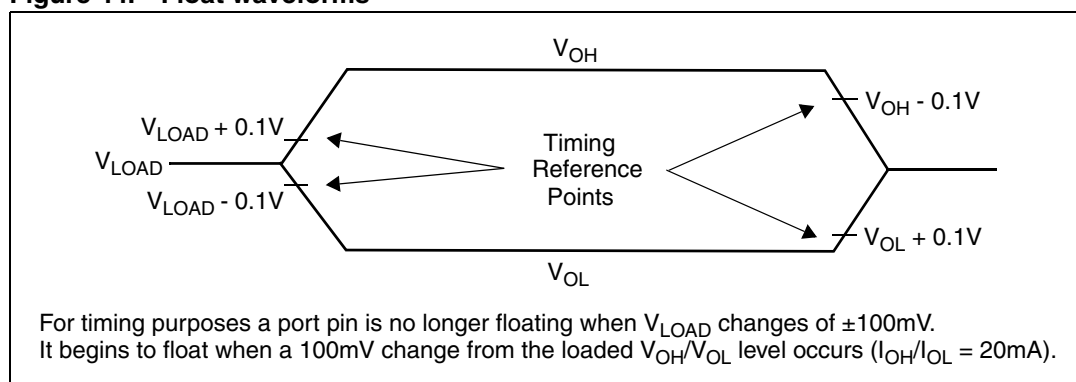
Figure 44. Float waveforms
