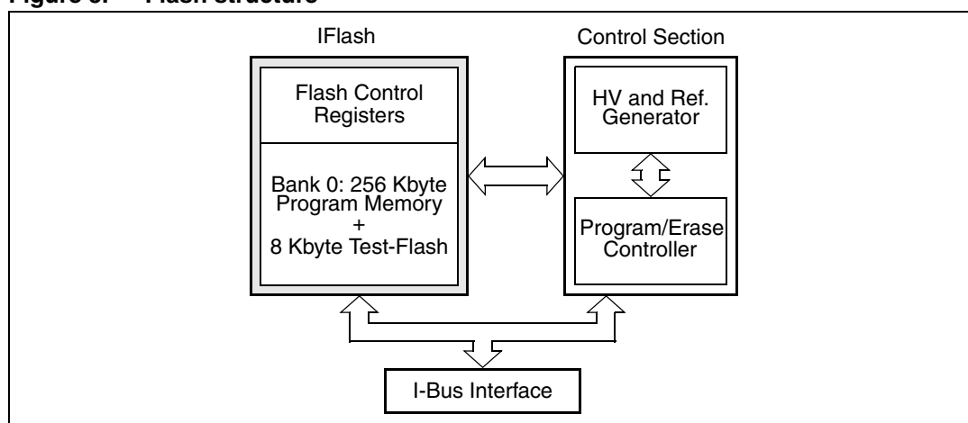
Figure 5. Flash structure
