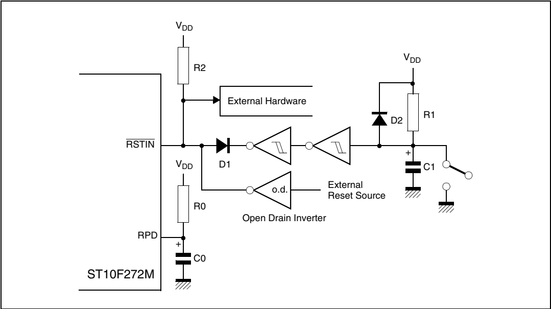
Figure 31. System reset circuit
