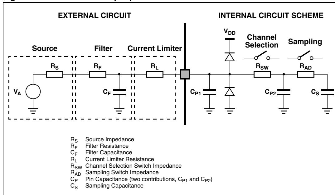
Figure 40. A/D converter input pins scheme
