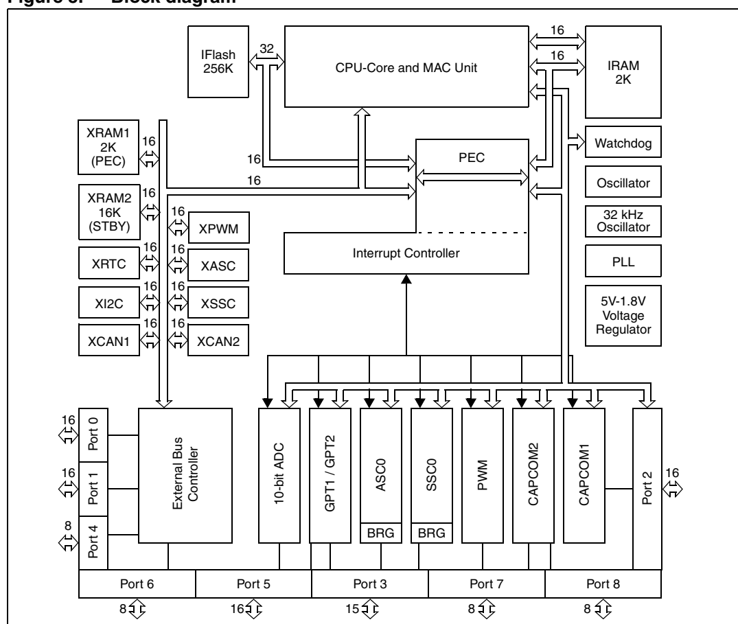
Figure 3. Block diagram
