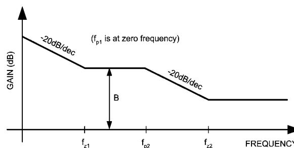
FIGURE 2. Output-Control Transfer Function
