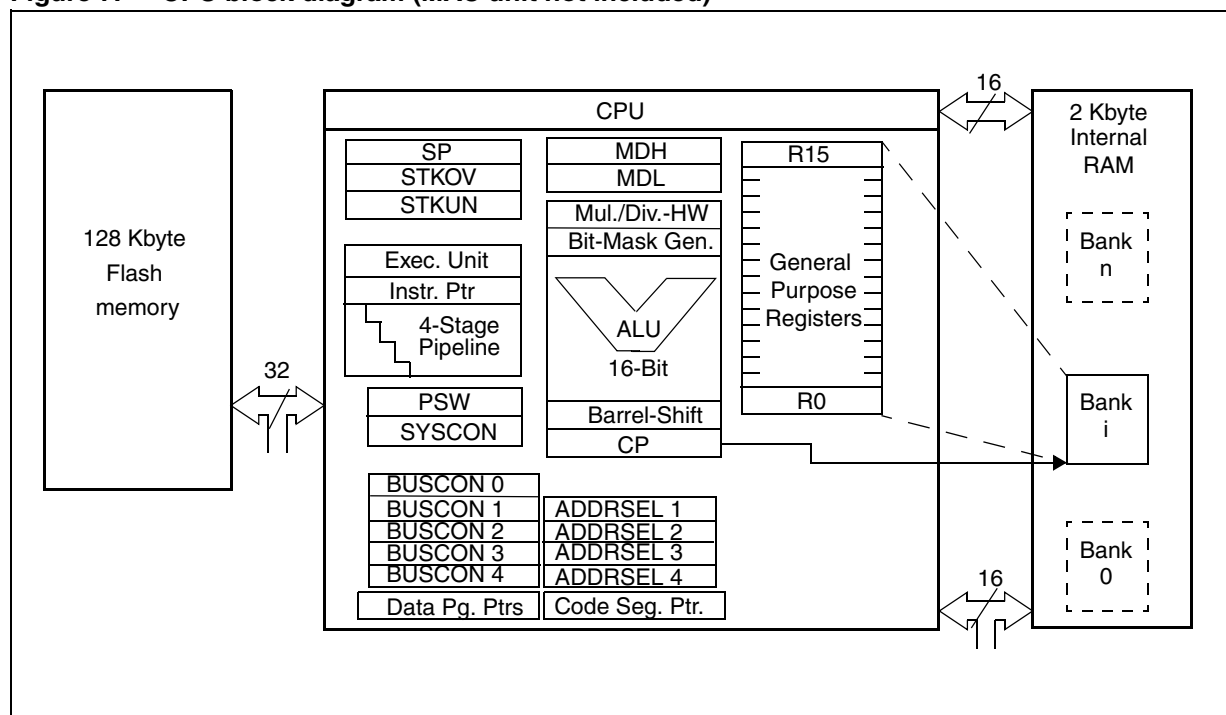
Figure 7. CPU block diagram (MAC unit not included)
