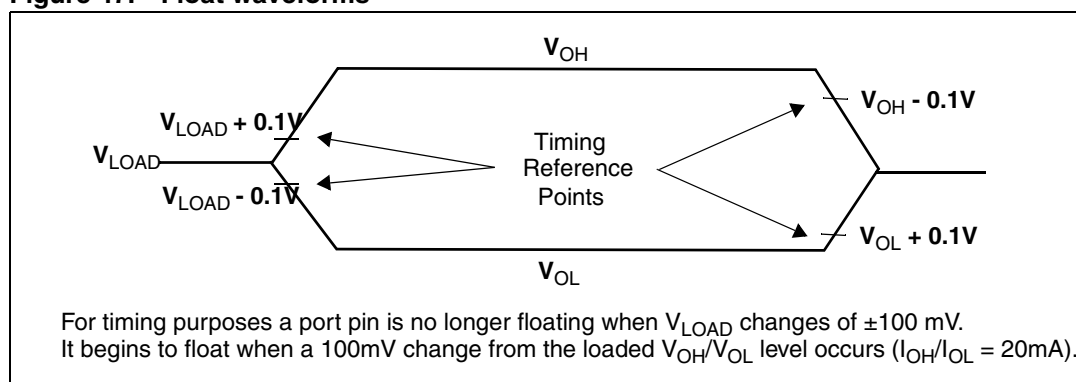
Figure 47. Float waveforms
