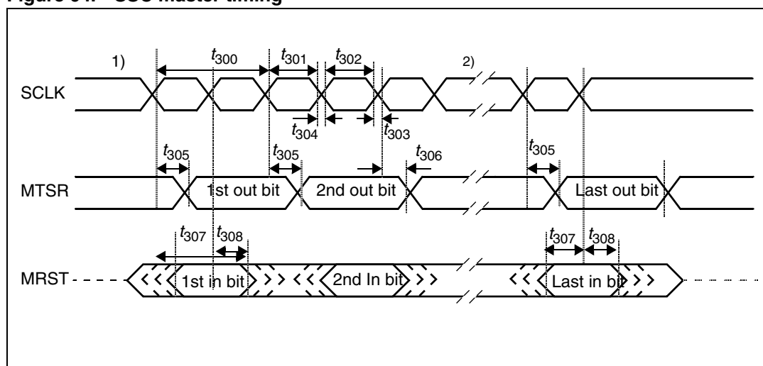
Figure 64. SSC master timing
