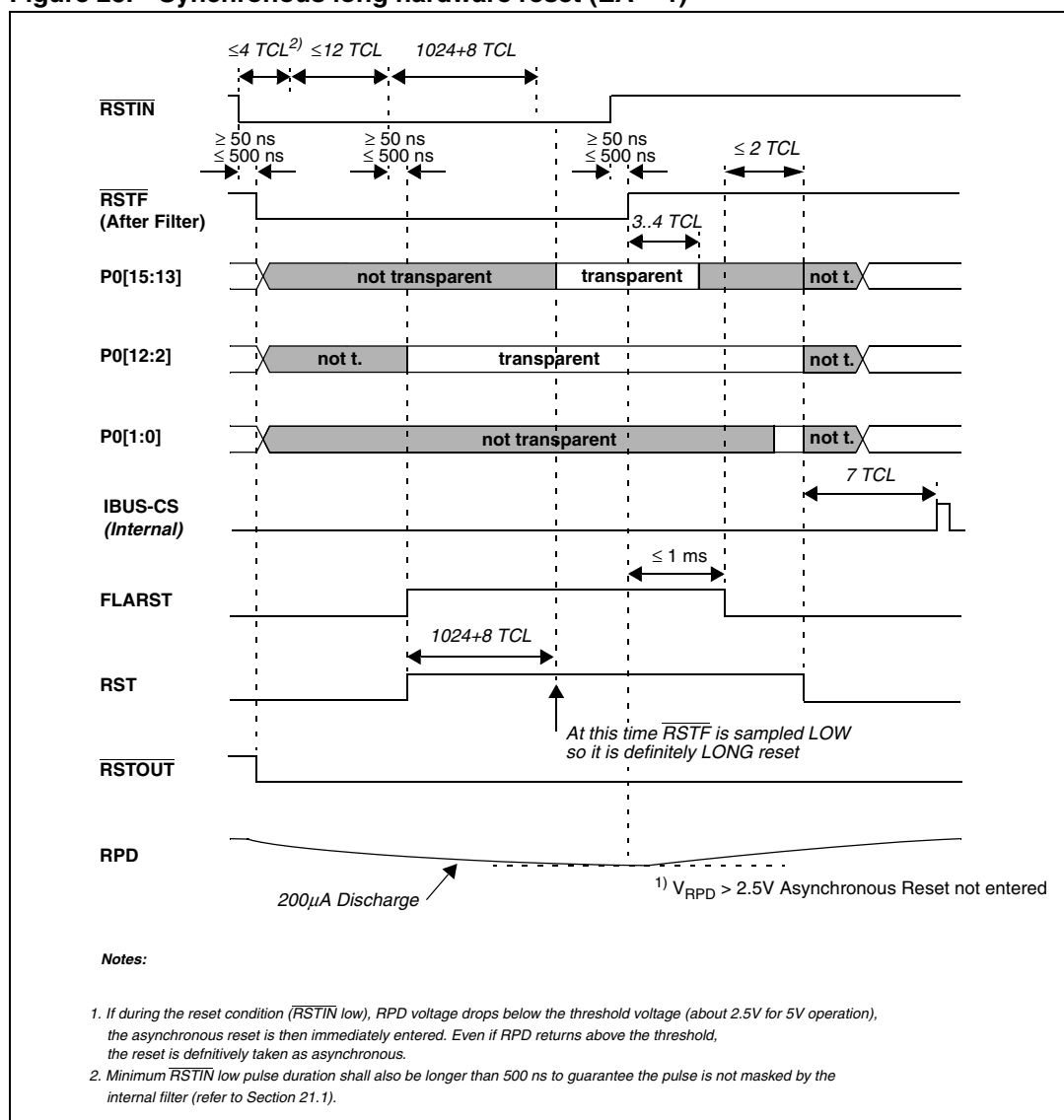
Figure 23. Synchronous long hardware reset ( \overline{\text{EA}} = 1 )
