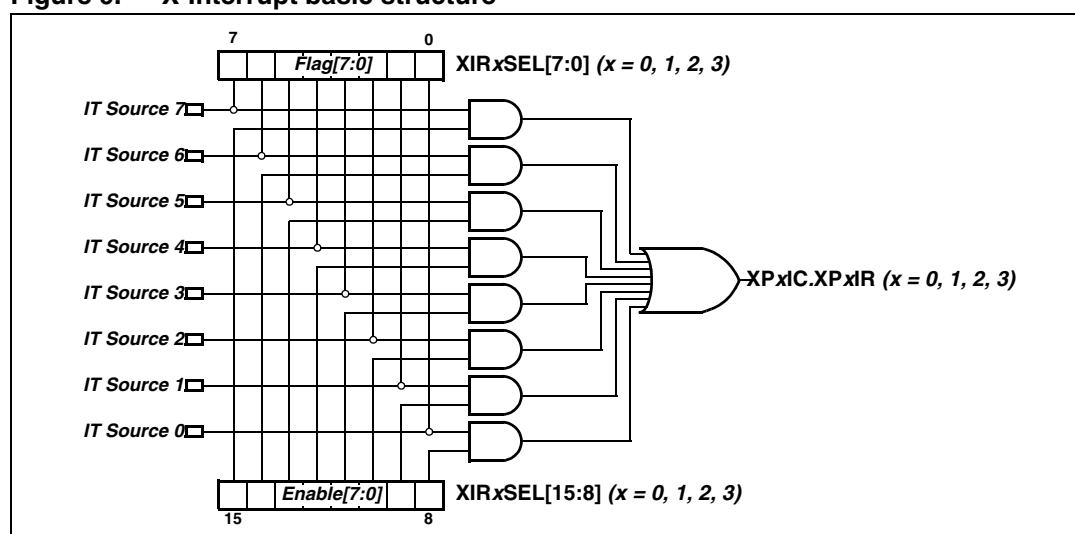
Figure 9. X-Interrupt basic structure
