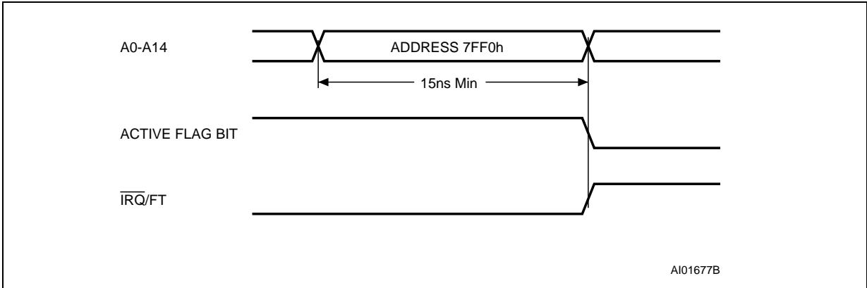
Figure 8. Alarm Interrupt Reset Waveform
