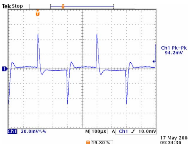
Figure 28. Transient Response without Optimal Voltage Positioning
