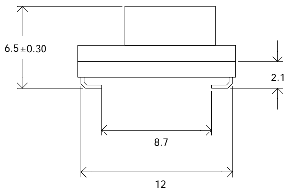
Figure 57. Side View
