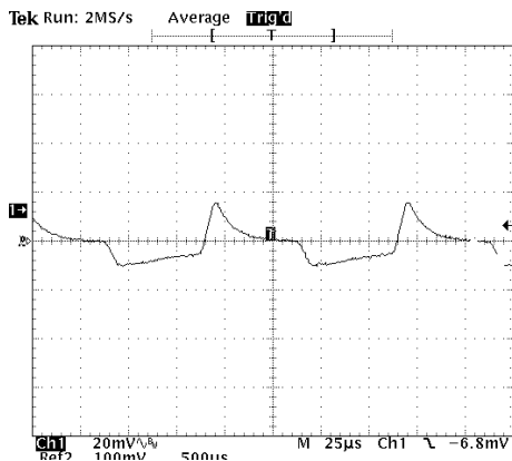
Load Transient
