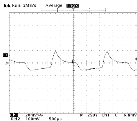
Load Transient
