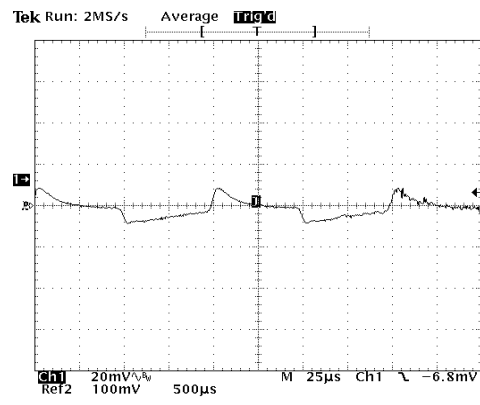
Load Transient
