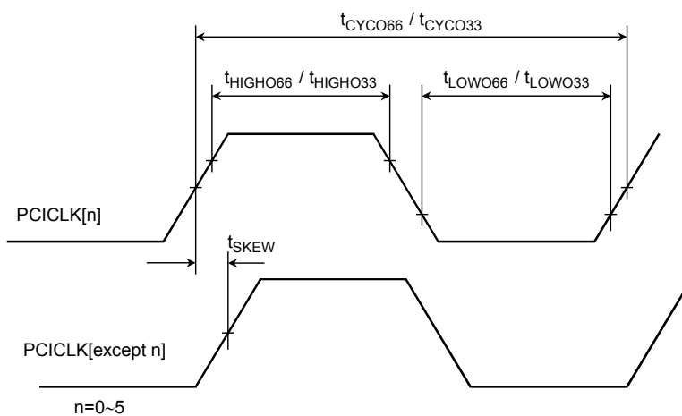
Figure 21.5.7 Timing Diagram: PCI Clock Skew
