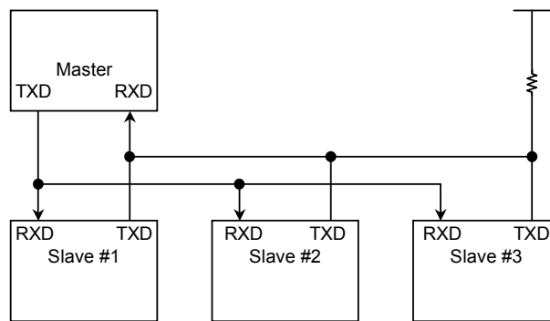
Figure 11.3.4 Example Configuration of Multi-Controller System
