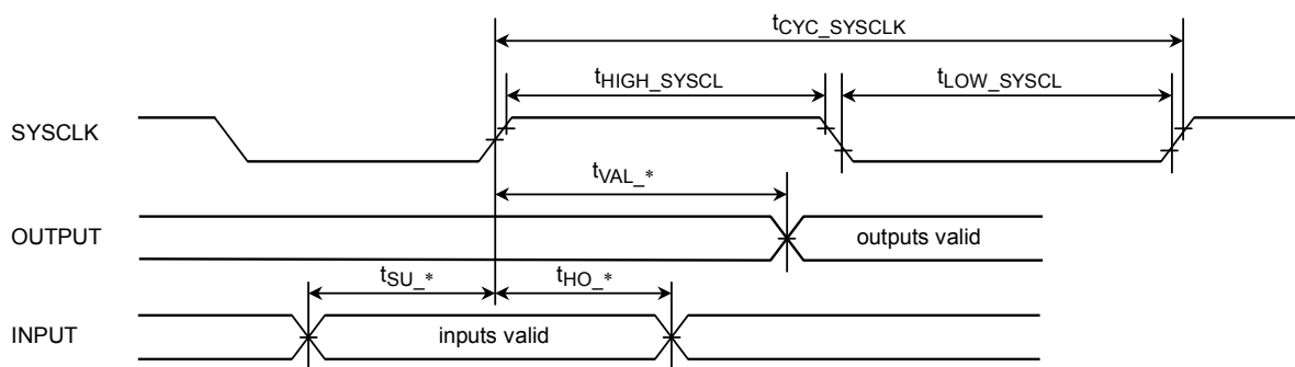
Figure 21.5.5 Timing Diagram: External Bus Interface
