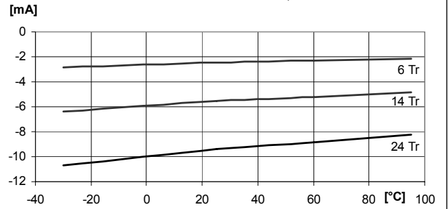
Port B: IOH current VDD=1.5V , VOH=1.2V
