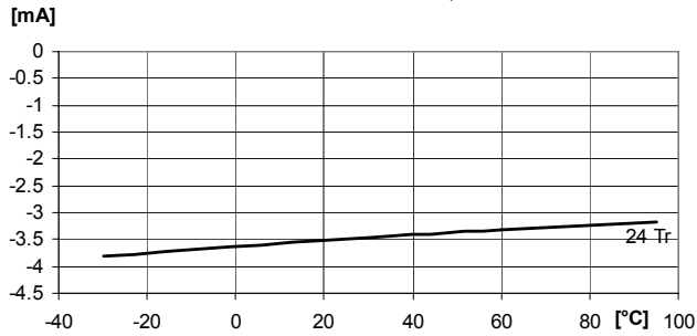
Port B: IOH current VDD=1.2V , VOH=1.05V
