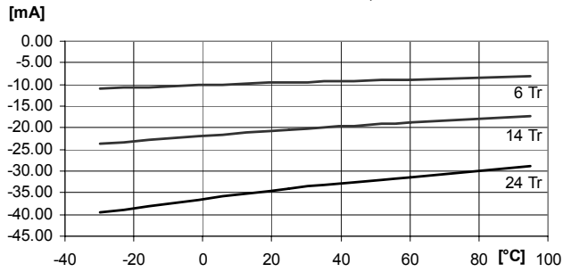
Port B: IOH current VDD=3.0V , VOH=2.5V
