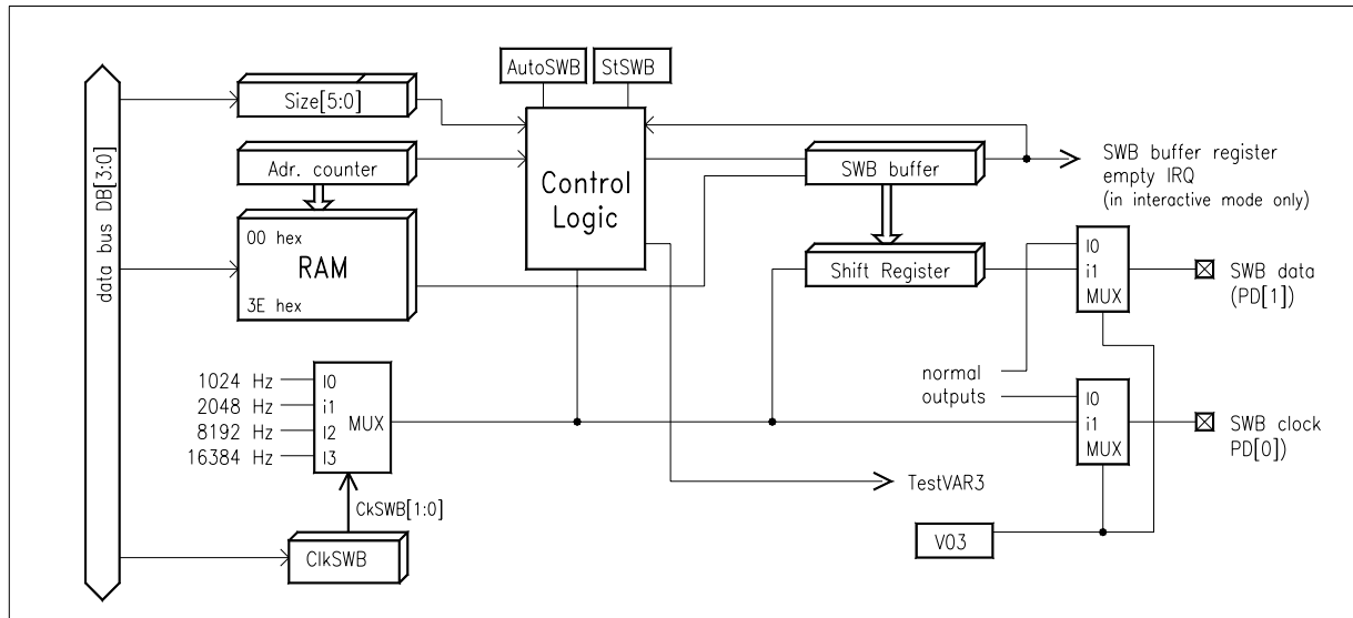
Figure 14. Serial write buffer
