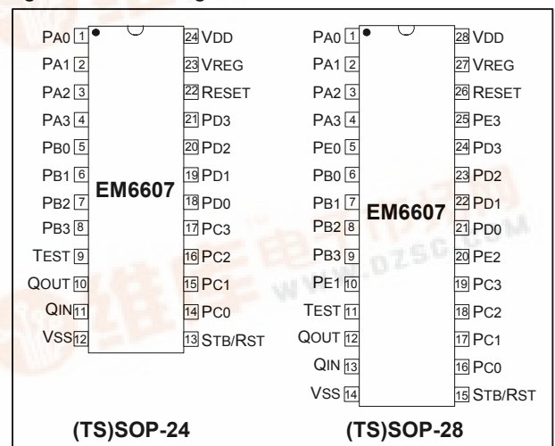
Figure 2. Pin Configuration
