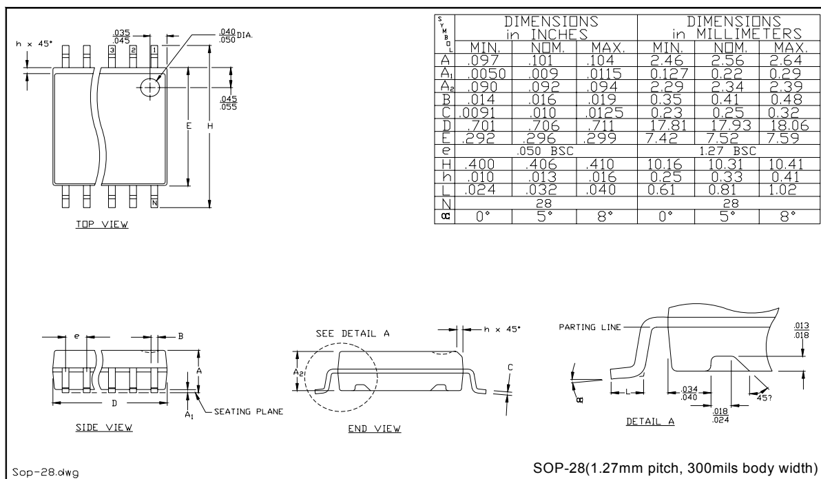
Figure 19. Dimensions of SOP28 Package SOIC
