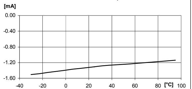
Port IOH current VDD=1.5V , VOH=1.2V
