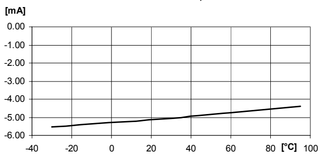
Port IOH current VDD=3.0V , VOH=2.5V
