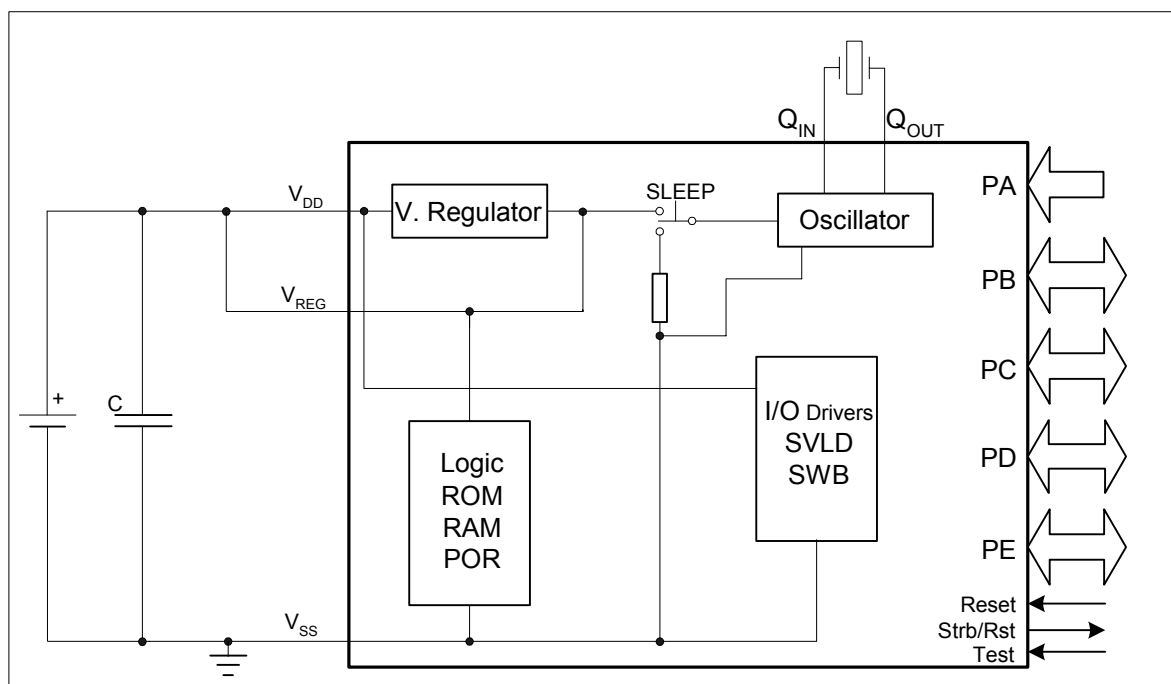
Figure 4. Typical Configuration: V_{DD} 1.2V up to 1.8V
