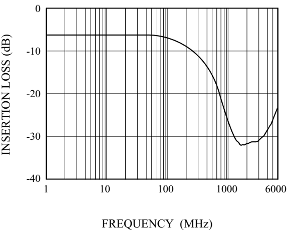
S_{21} - F
