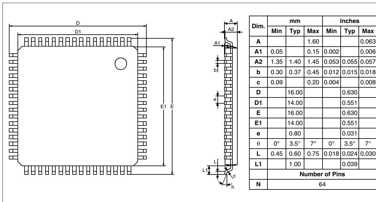
Figure 163. 64-Pin Low Profile Quad Flat Package (14x14)
