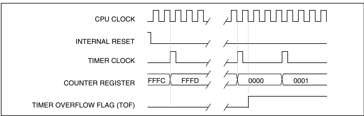
Figure 46. Counter Timing Diagram, internal clock divided by 4
