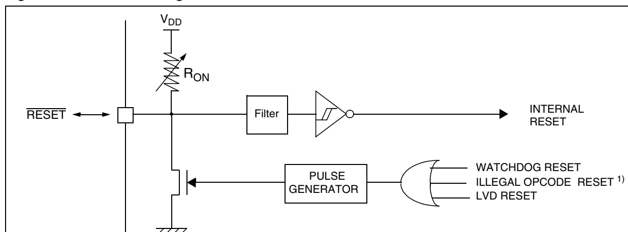
Figure 15. Reset Block Diagram
