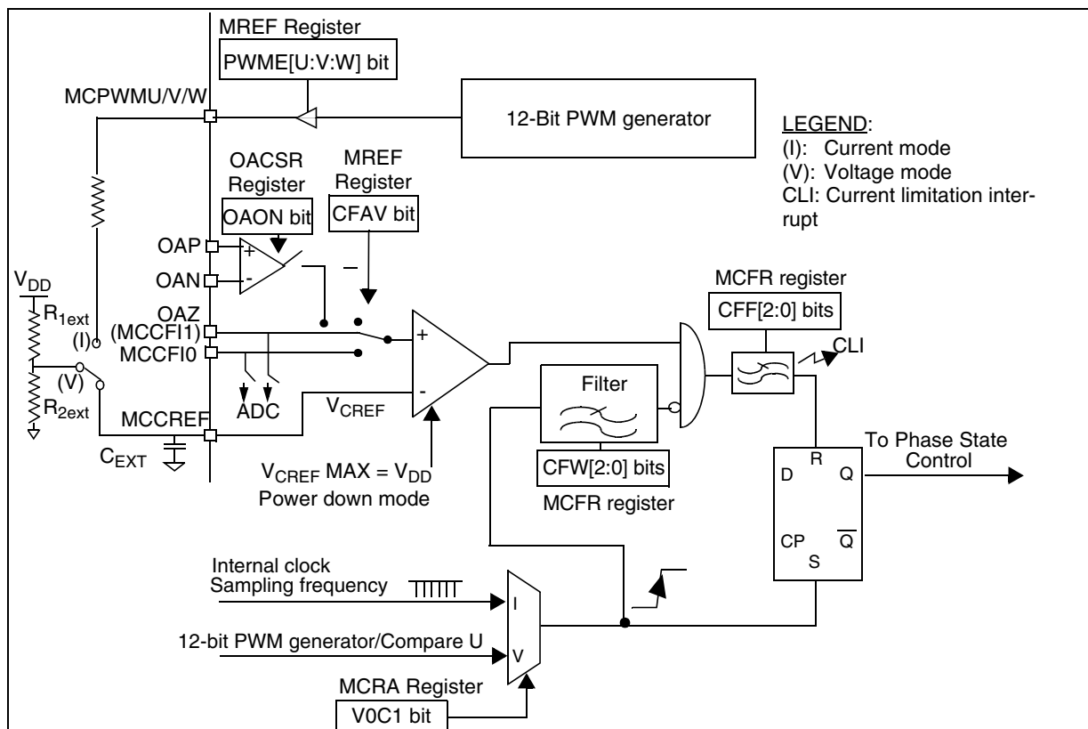
Figure 106. Current Feedback
