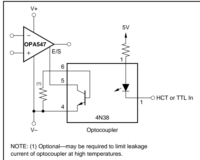
FIGURE 6. Output Disable with Dual Supplies.
