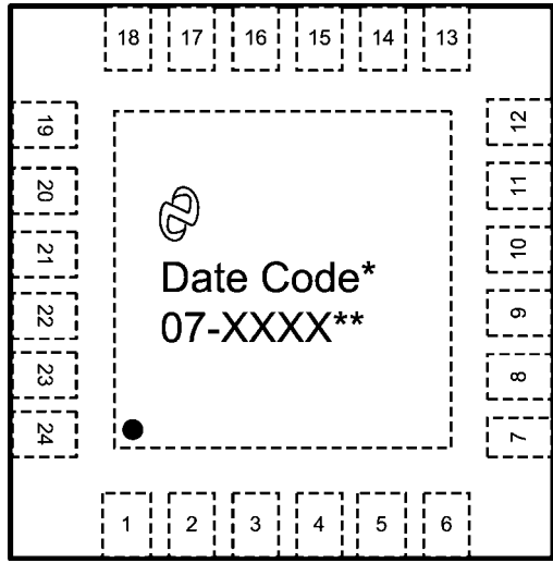
FIGURE 3. 24-Lead LLP Package (Top View)
