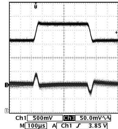
Line Transient (LDO2) 3 - 4.2\text{V}_{IN} , 3.3\text{V}_{OUT} , 300 mA load
