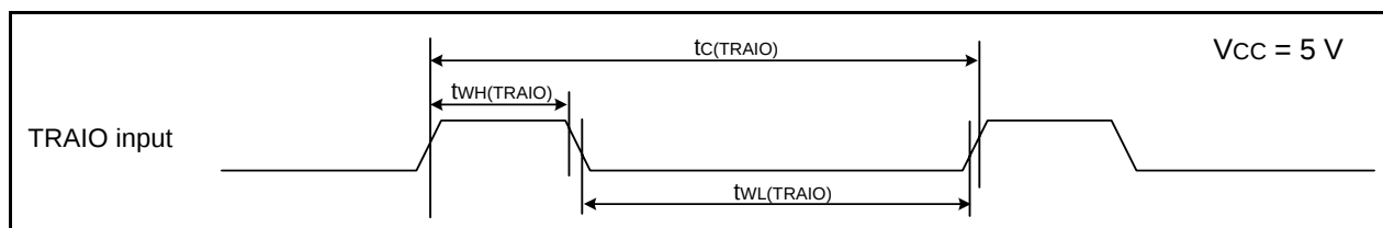
Figure 5.9 TRAIO Input and INT1 Input Timing Diagram when V_{CC} = 5\text{ V}
