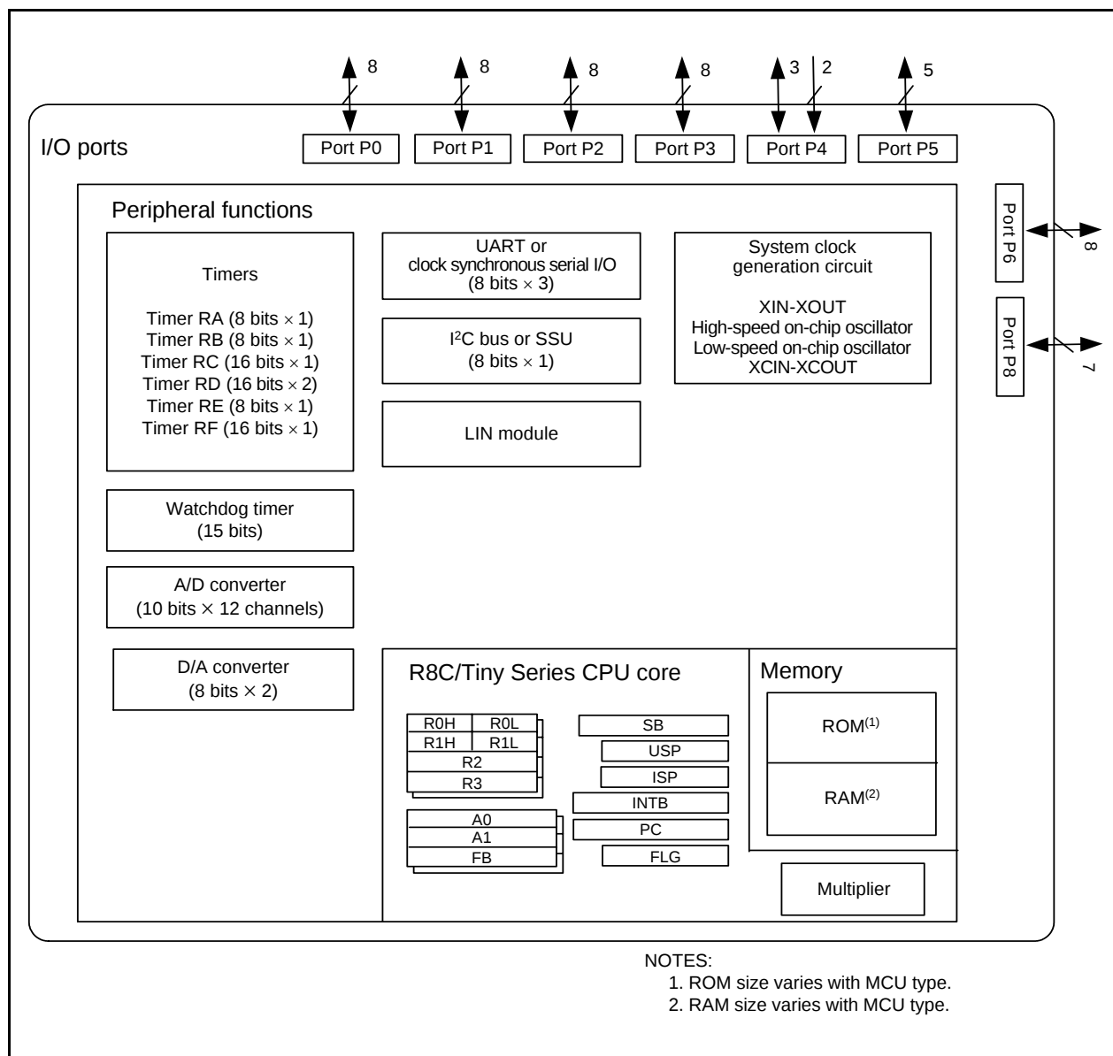
Figure 1.3 Block Diagram
