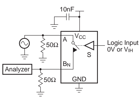
Figure 11. Off Isolation
