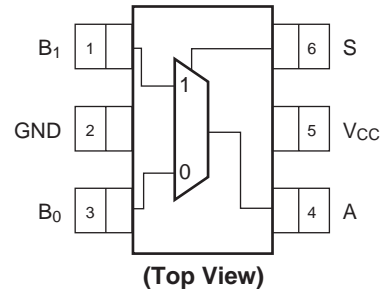
Pin Assignments for SC70
