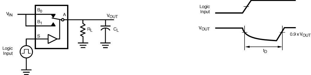
FIGURE 3. Break Before Make Interval Timing
