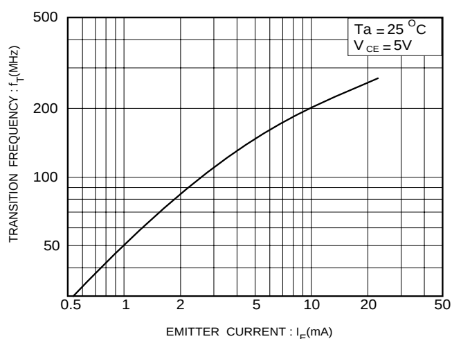
Fig.6 Gain bandwidth product vs. emitter current
