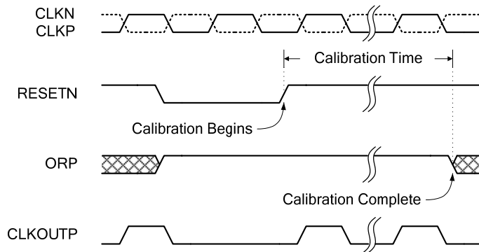
Figure 29. Calibration Timing
