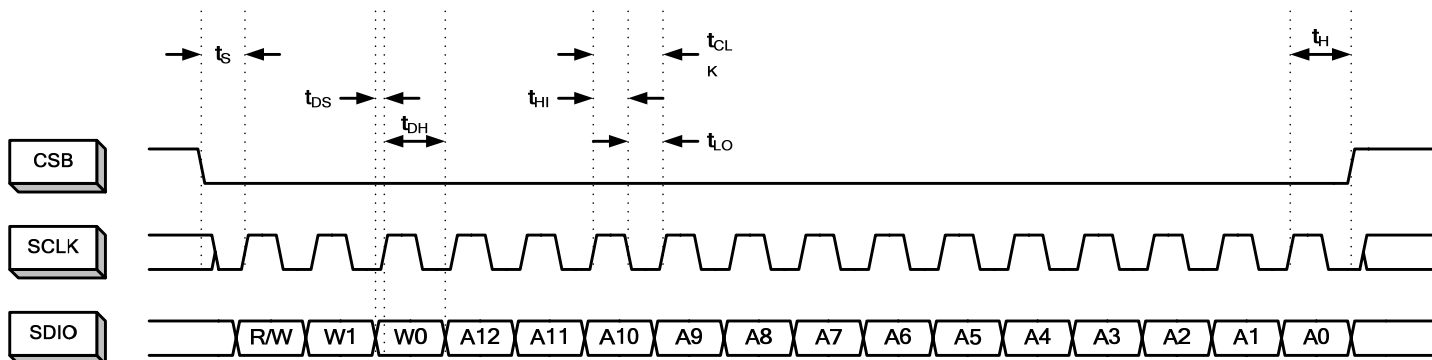
Figure 42. Instruction/Address Phase
