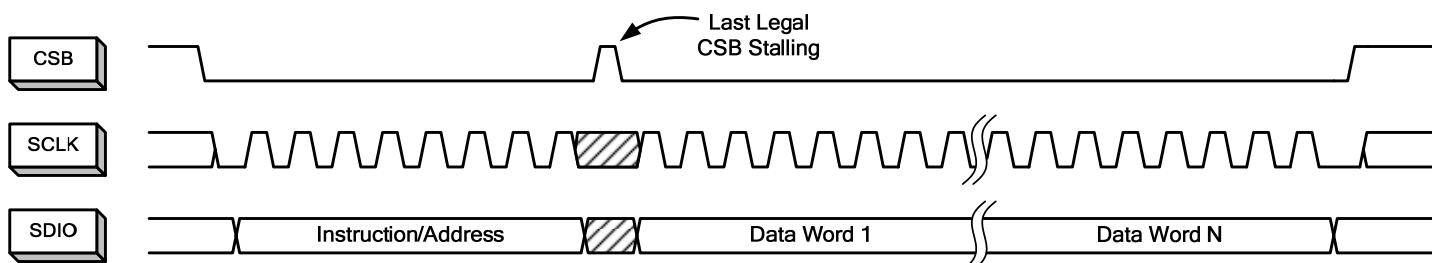
Figure 44. N-Byte Transfer
