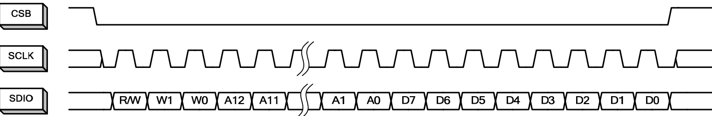
Figure 40. MSB-First Addressing
