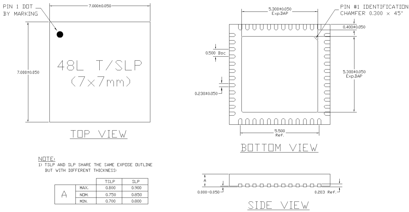
Figure 55. 48QFN Dimensions
