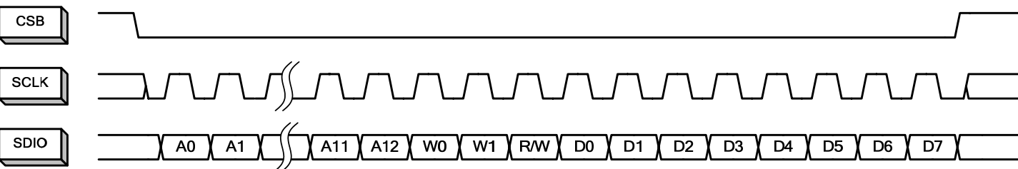
Figure 41. LSB-First Addressing
