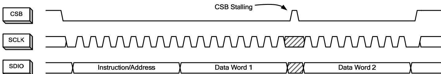
Figure 43. 2-Byte Transfer
