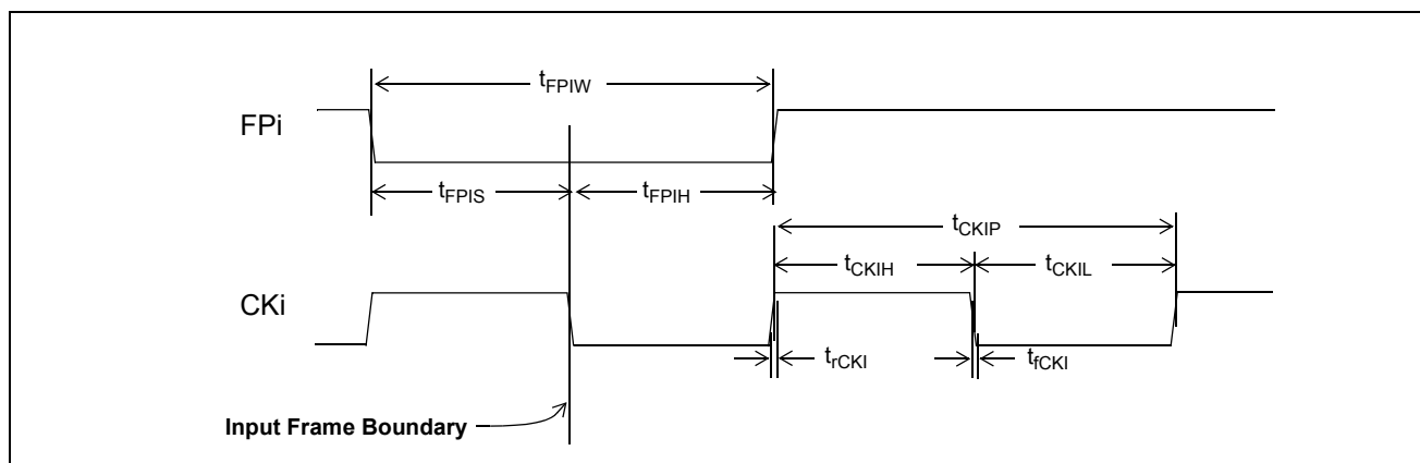
Figure 20 - Frame Pulse Input and Clock Input Timing Diagram (ST-BUS)
