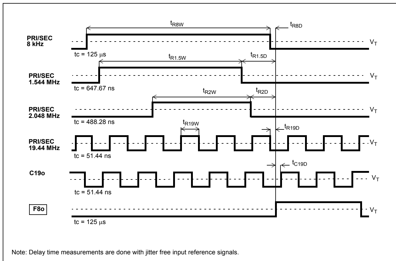
Figure 21 - Input Reference to Output Clock Phase Offset
