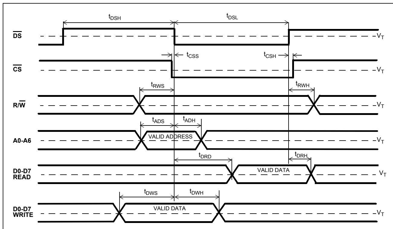
Figure 17 - Microport Timing
