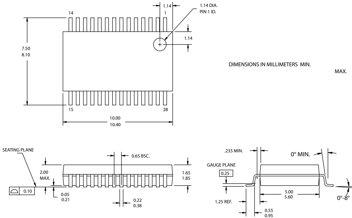
28-Lead (5.3 mm) Shrink Small Outline Package O28
