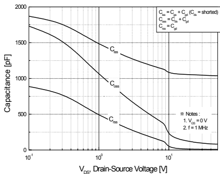
Figure 5. Capacitance Characteristics
