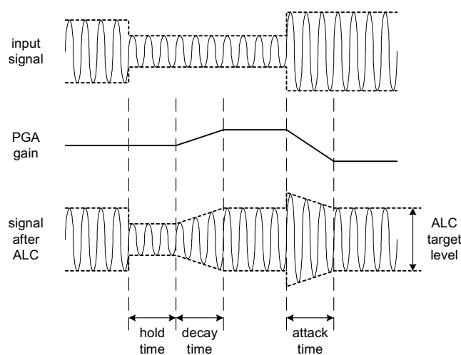
Figure 10 ALC Operation
