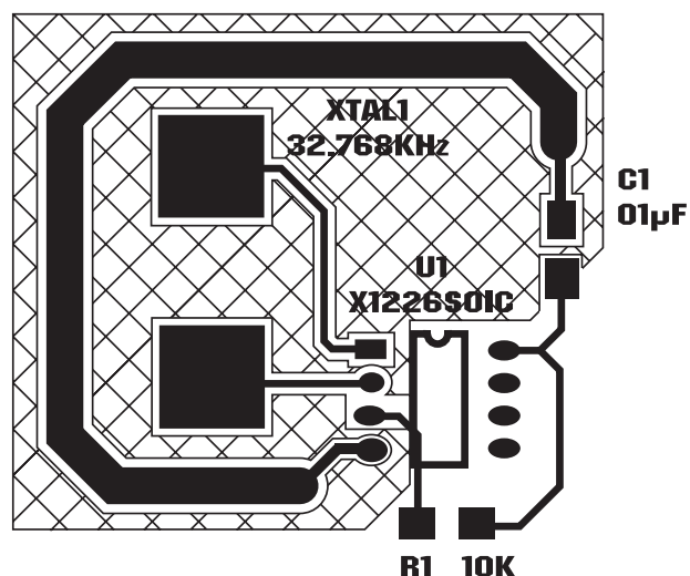
FIGURE 27. SUGGESTED LAYOUT FOR INTERSIL RTC IN SO-8
