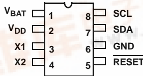
ISL12027 (8 LD TSSOP) TOP VIEW
