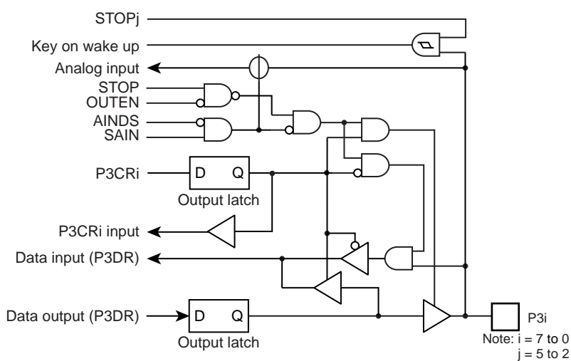
Figure 5-5 Port P3
