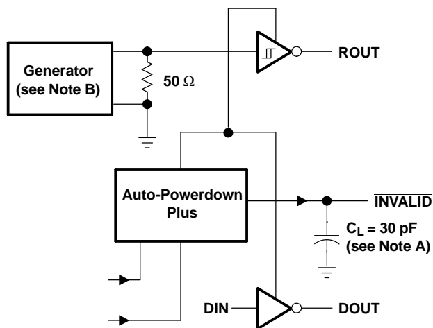
Figure 4. \overline{\text{INVALID}} Propagation Delay Times and Driver Enabling Time
